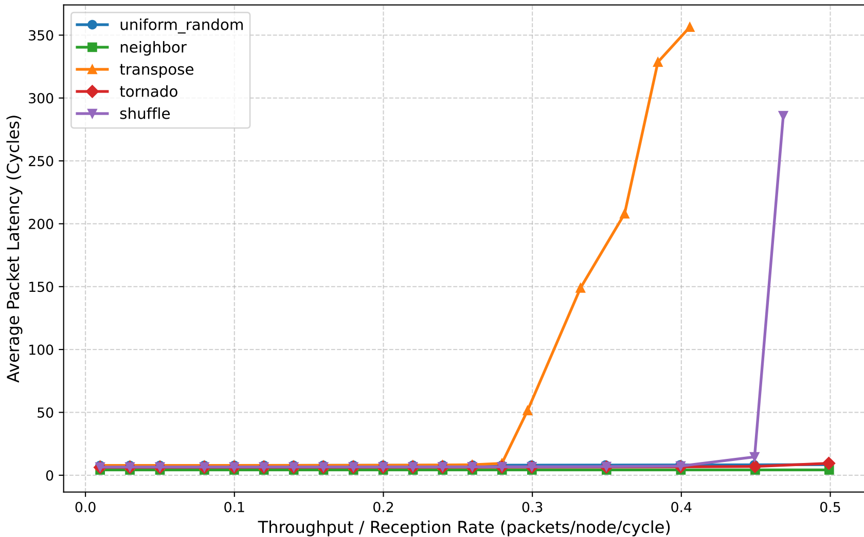
Latency vs Throughput (8x8 Mesh, 10,000 Cycles)
