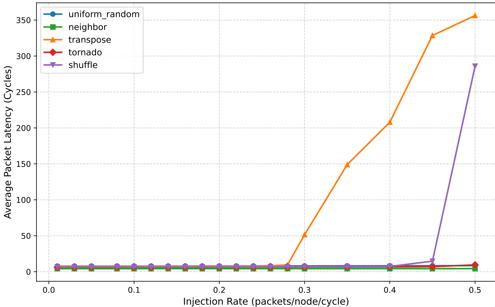
Latency vs Injection Rate (8x8 Mesh, 10,000 Cycles)
