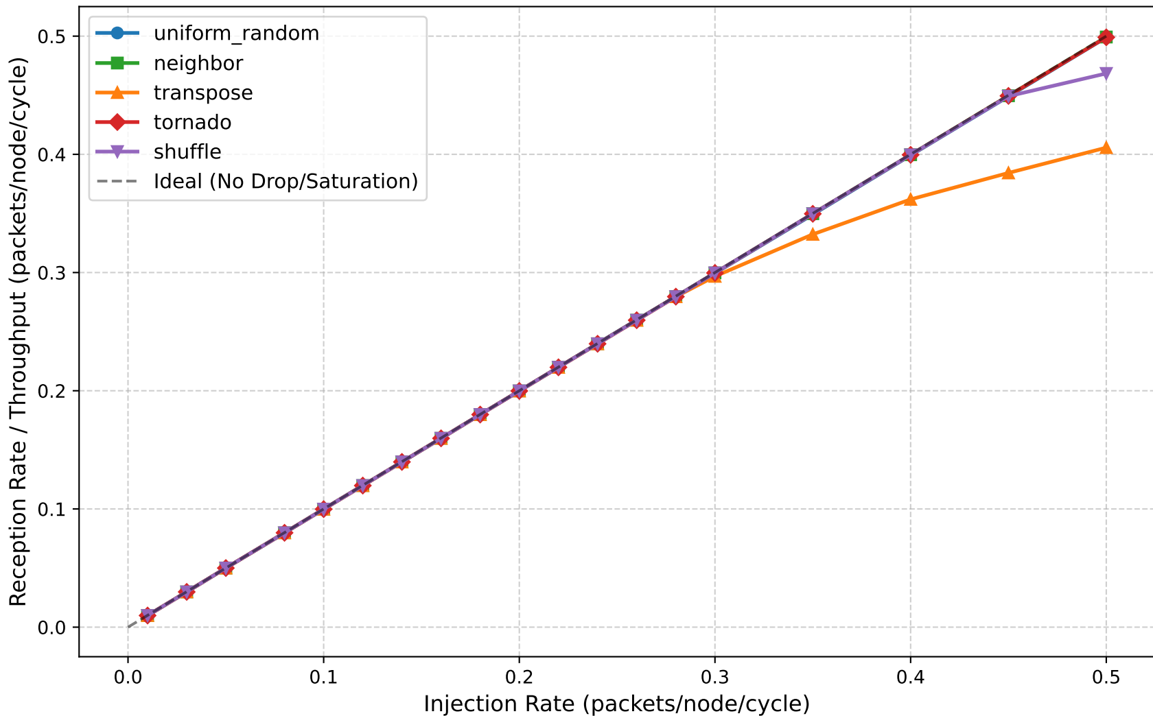
Throughput vs Injection Rate (8x8 Mesh, 10,000 Cycles)
