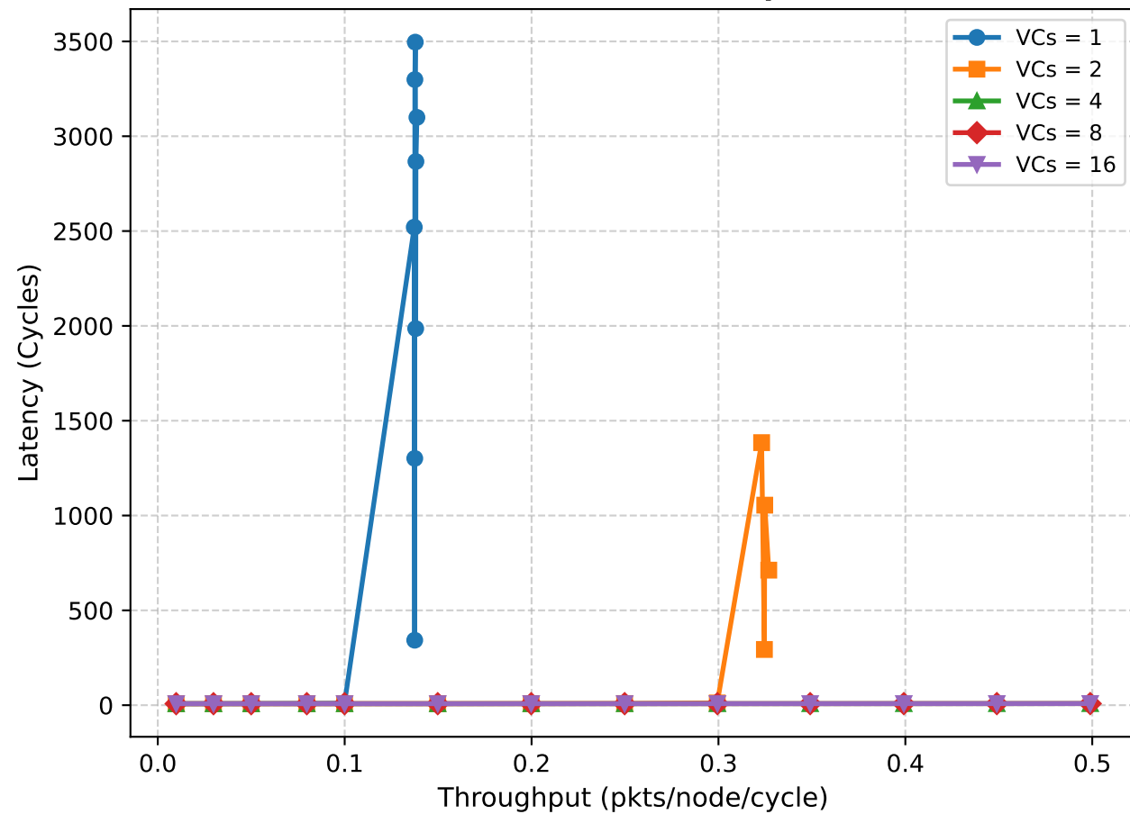
(a) Virtual Channels (vcs-per-vnet)
