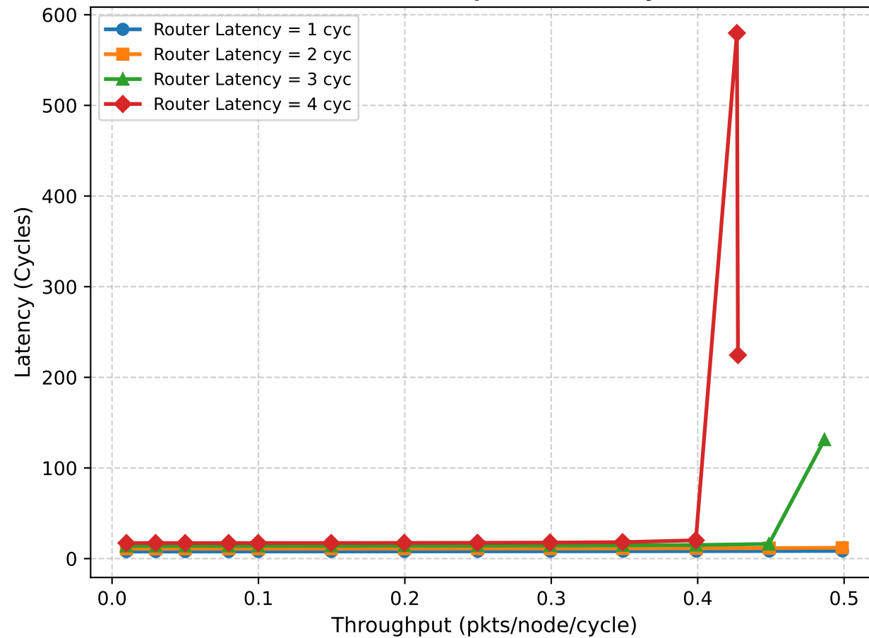
(b) Router Pipeline Latency
