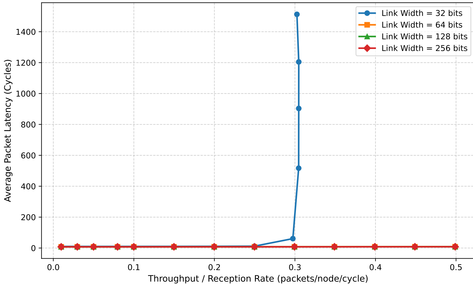
Impact of Physical Link Width on Latency-Throughput (8x8 Mesh)
