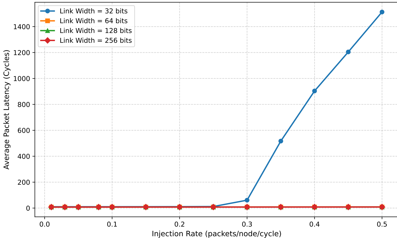
Impact of Physical Link Width on Latency vs. Injection Rate
