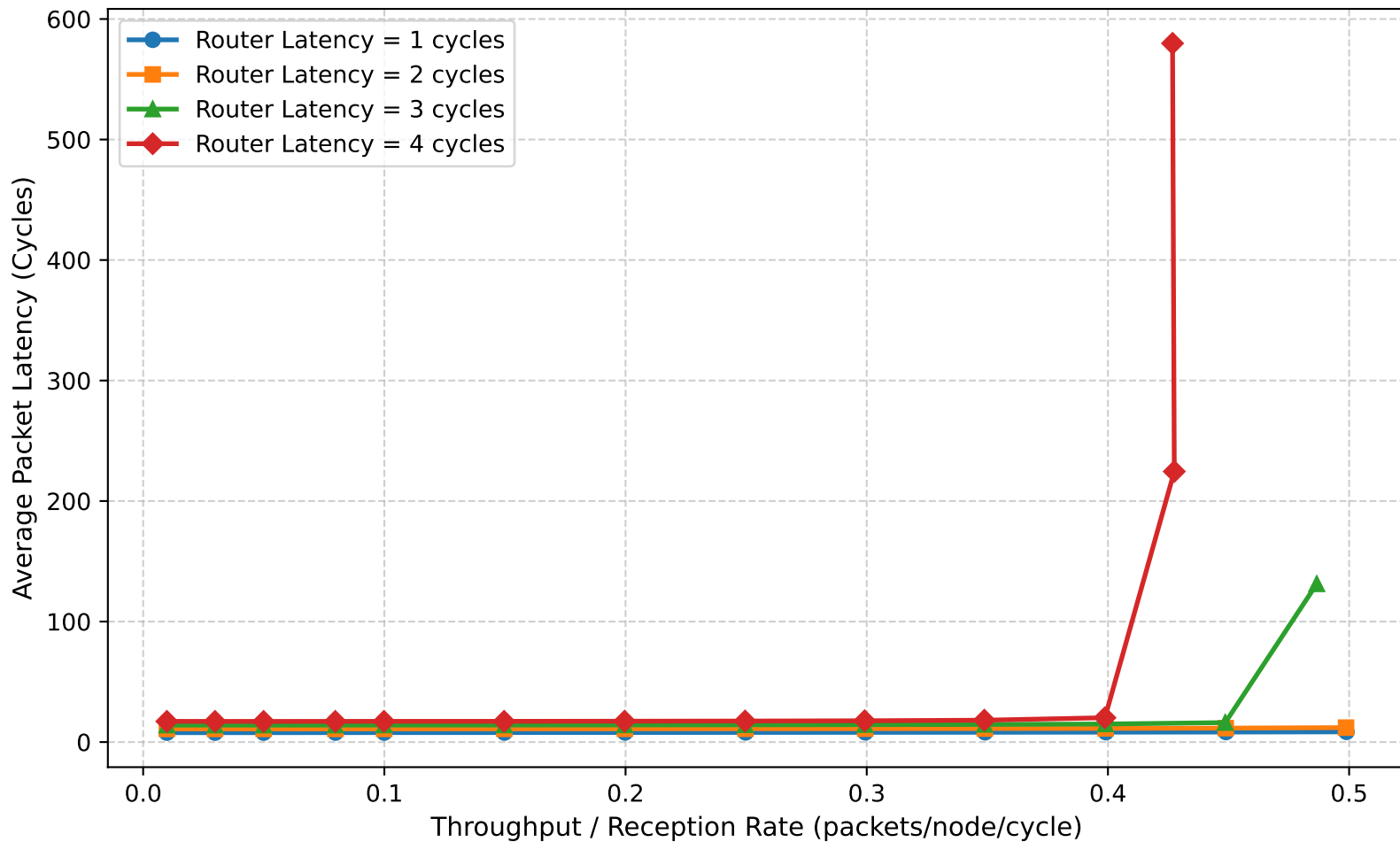
Impact of Router Pipeline Latency on Latency-Throughput (8x8 Mesh)
