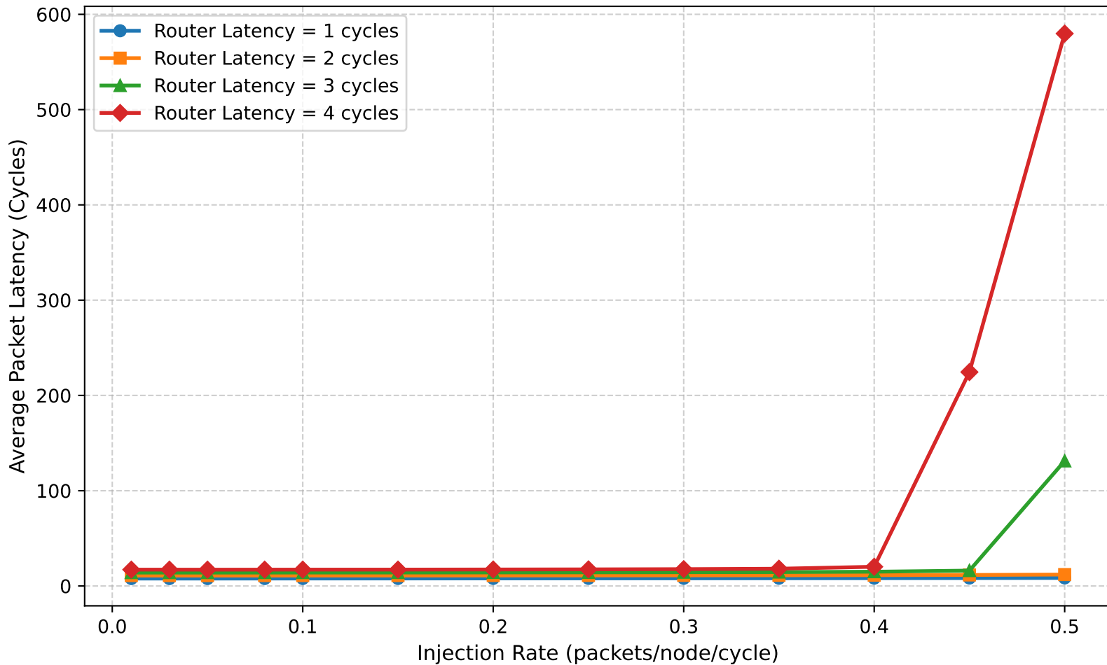
Impact of Router Pipeline Latency on Latency vs. Injection Rate
