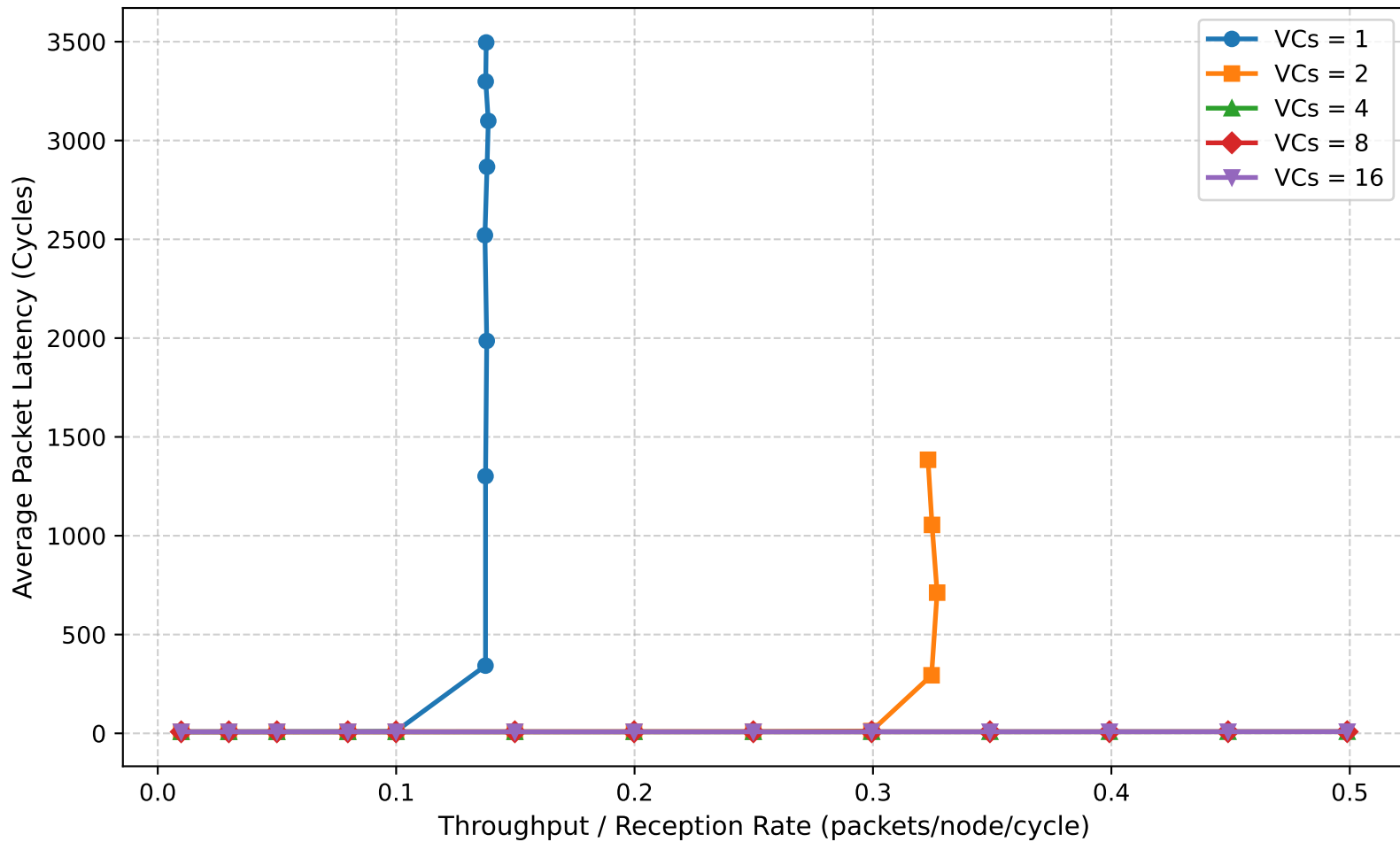
Impact of Virtual Channel Count on Latency-Throughput (8x8 Mesh)
