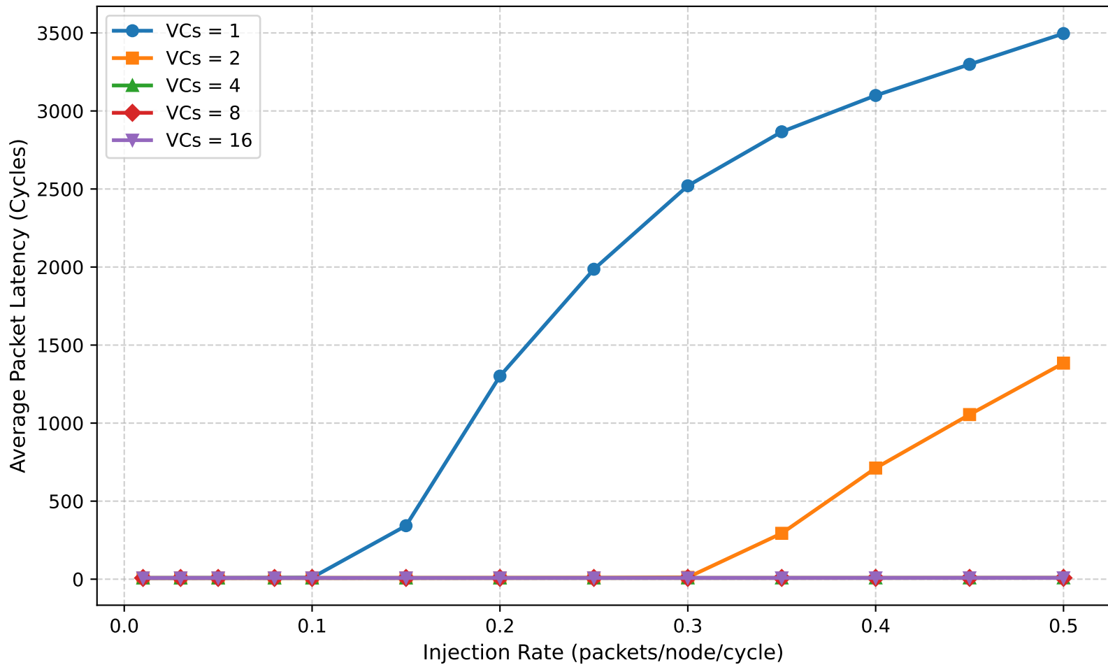
Impact of Virtual Channel Count on Latency vs. Injection Rate
