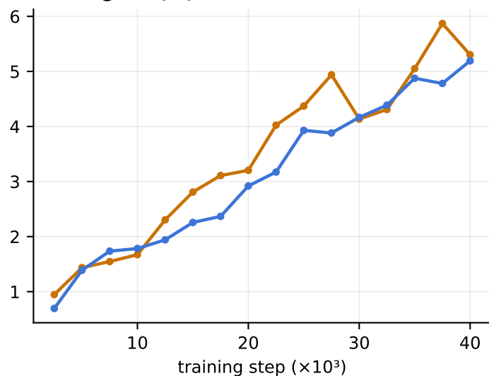
Recall@1 ↑ (%)
