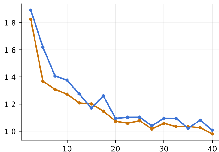
Recall@5 ↑ (%)
