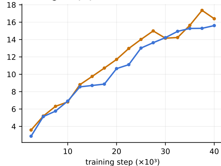
Recall@5 ↑ (%)
