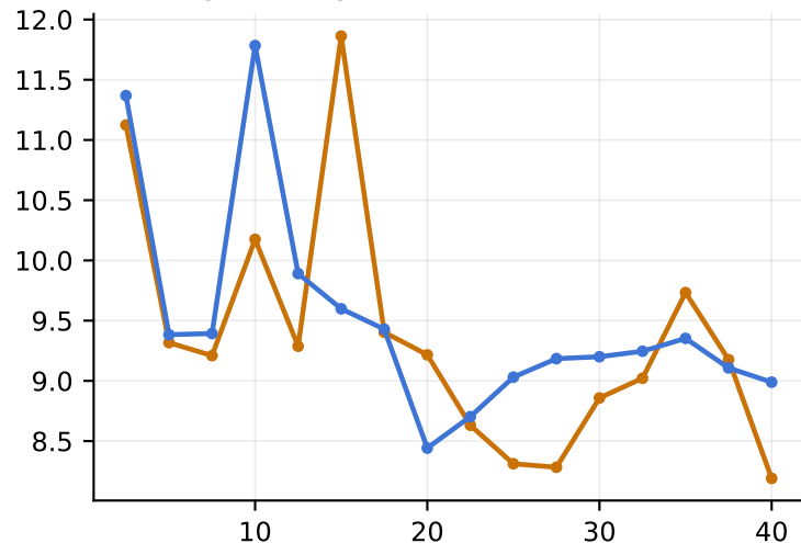
Recall@1 ↑ (%)
