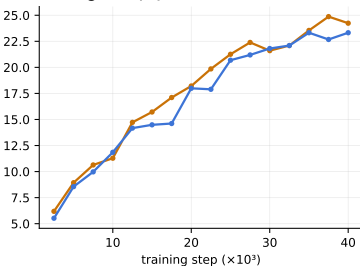
Recall@10 ↑ (%)
