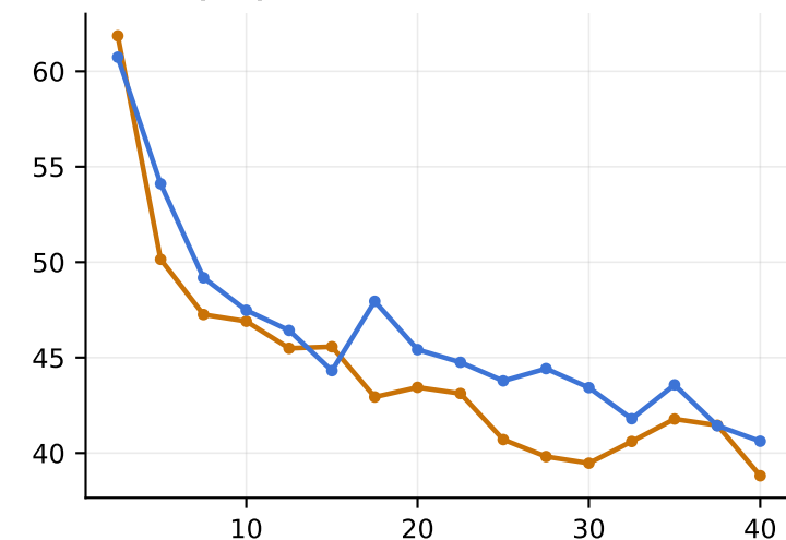
Recall@10 ↑ (%)
