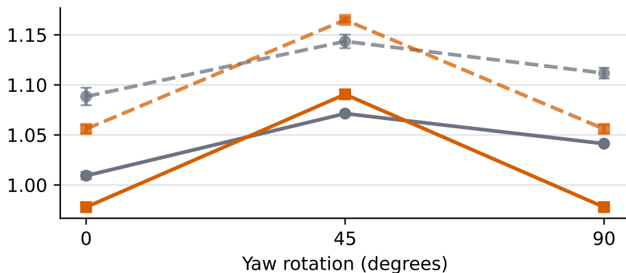
C50 error (dB) \downarrow
