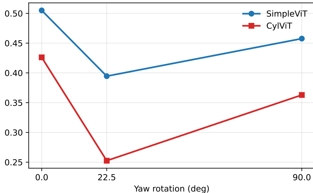
RIR-to-GT R@10 (%) (higher is better)
