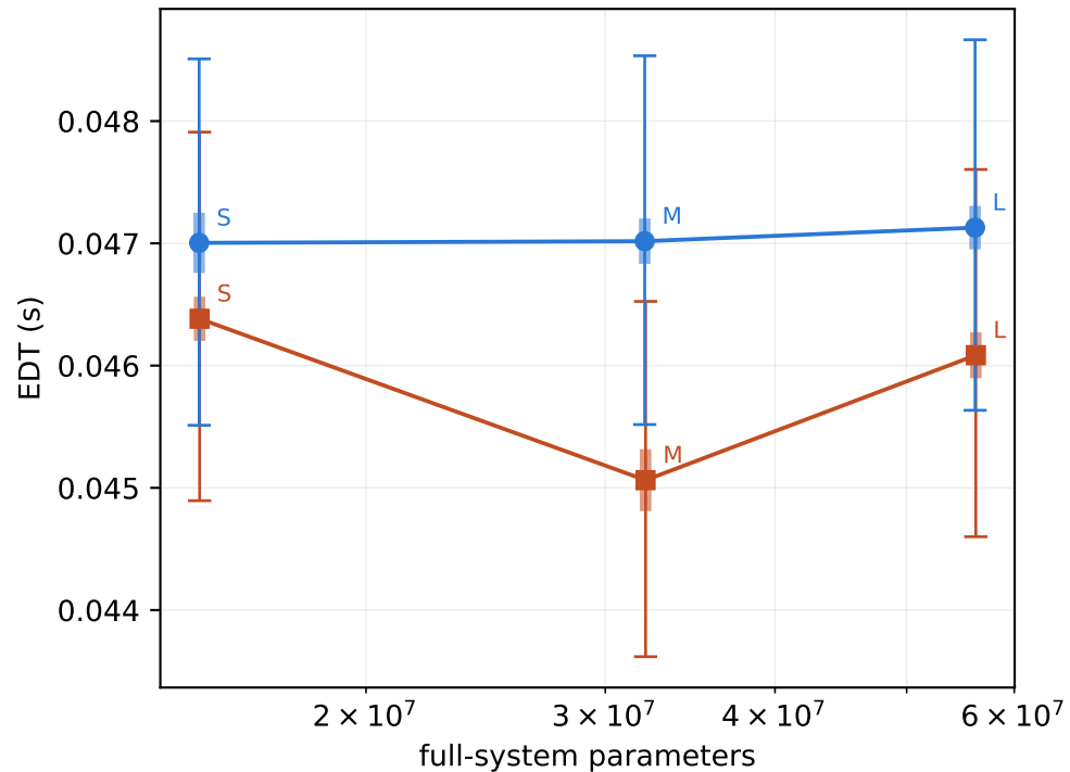
CURVE_K8 — EDT against capacity (K = 8, five seeds, own cohorts)
