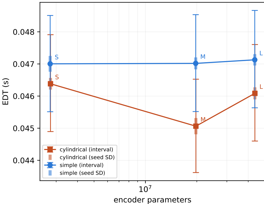
CURVE_K8 — EDT against capacity (K = 8, five seeds, own cohorts)
