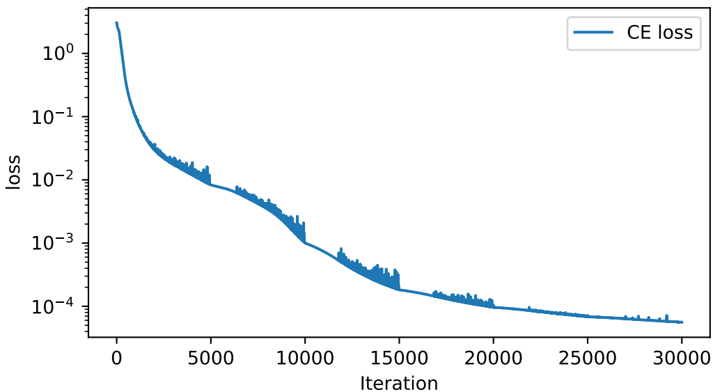
Cross Entropy loss with LSTM on tiny_extract_m404 H=1.6156
