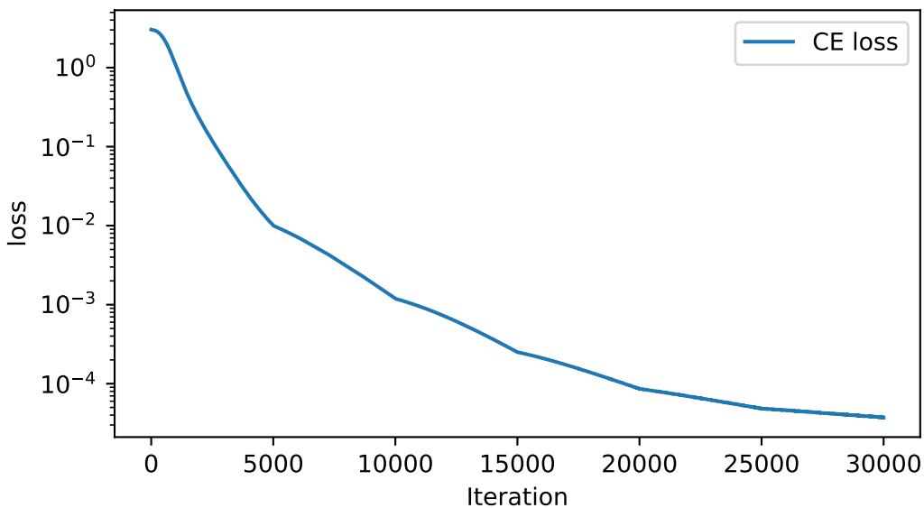
Cross Entropy loss with UFM on tiny_extract_m404 H=1.6156
