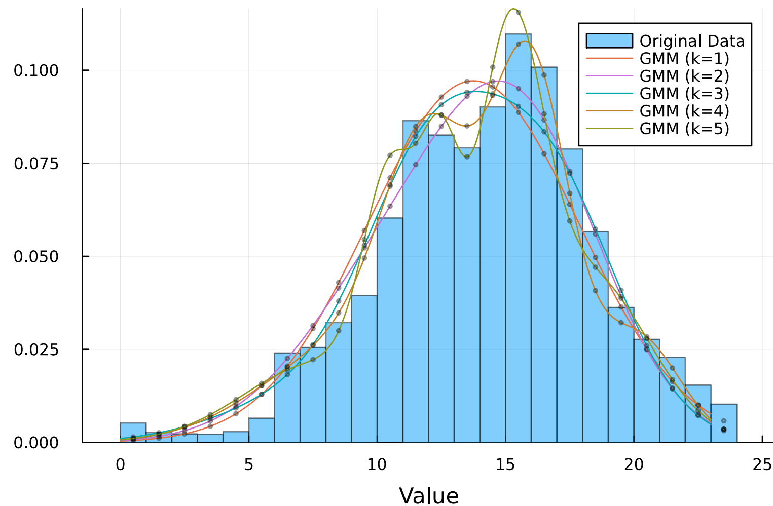
Original and GMM Modeling: Energy Demand
