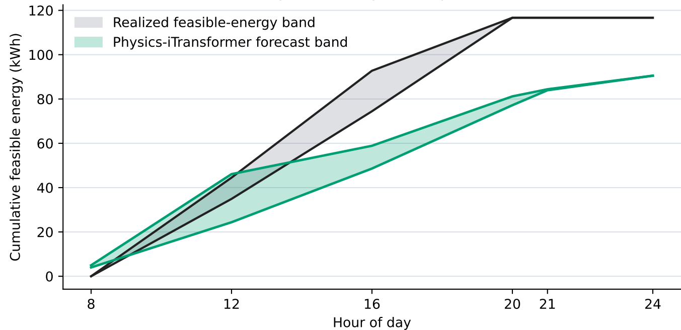
Full six-charger flexibility envelope: 2023-09-06
