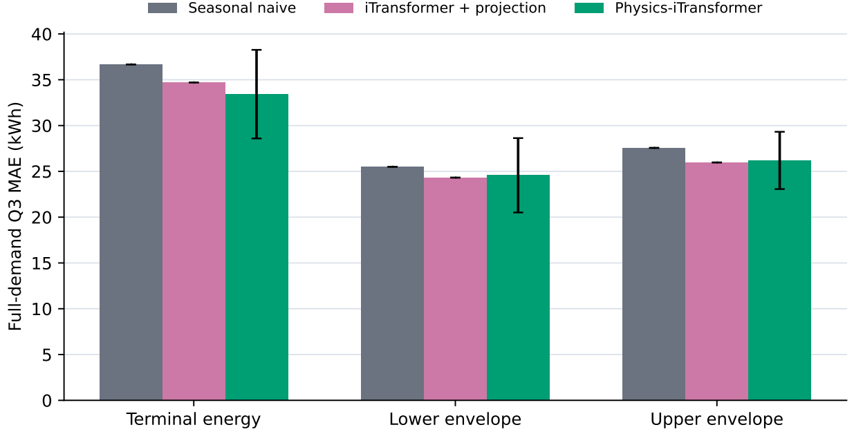
Figure 6: Full-demand Q3 flexibility error. Physics-iTransformer improves all three mean errors over seasonal naive, but individual seeds do not uniformly beat that deterministic baseline.
