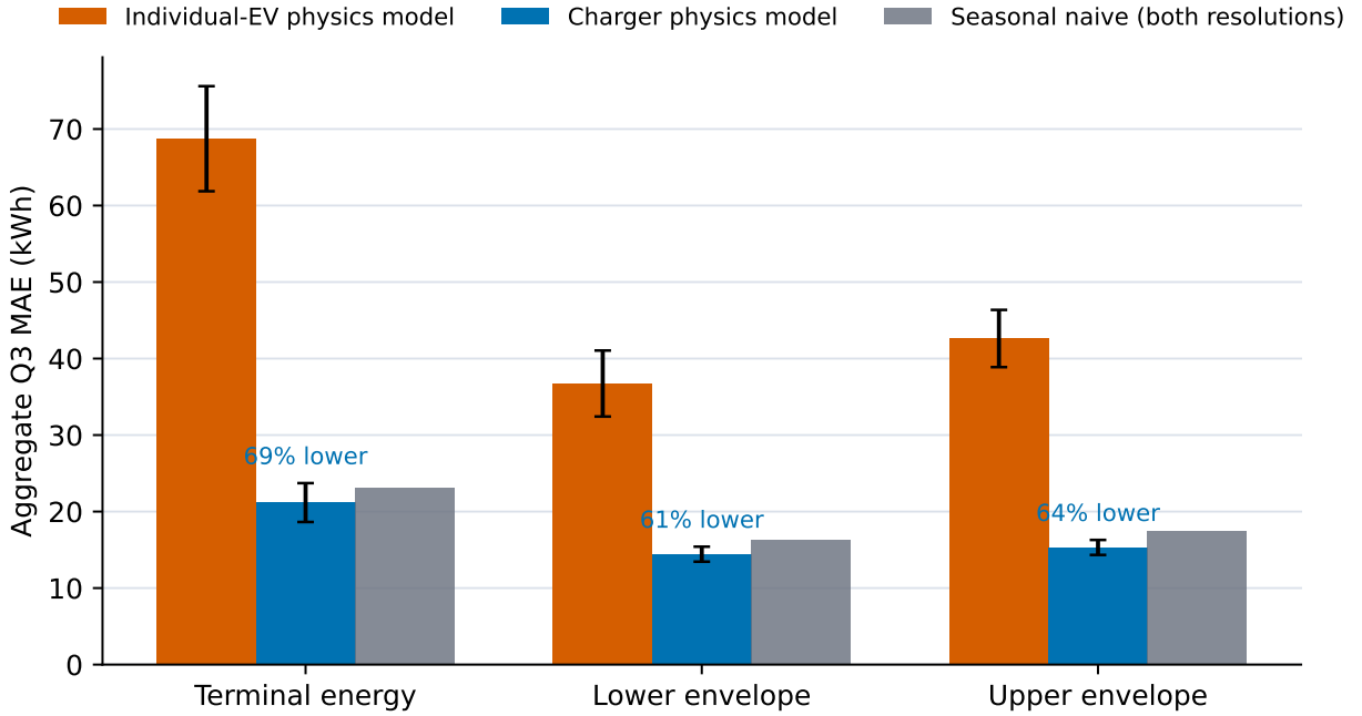
Figure 4: Physics-constrained forecast error on identical realized flexibility signatures. Error bars are seed standard deviations. The seasonal-naive bar is shared by EV and charger resolutions because lag and aggregation commute.
