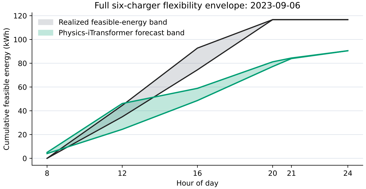
Figure 7: Representative full-demand day selected by median three-seed terminal error. Filled regions show realized and physics-iTransformer cumulative feasible-energy bands at the six anchors. Both predicted curves satisfy the physical cone despite the terminal-energy forecast error.
