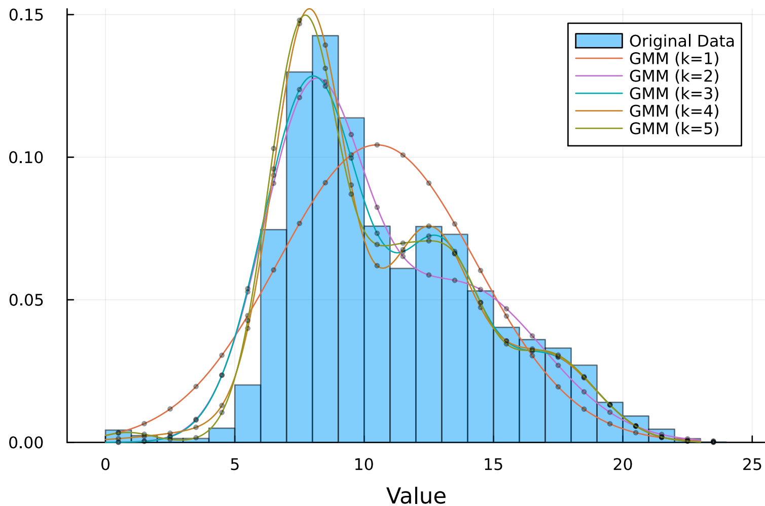
Original and GMM Modeling: Plug-in Duration
