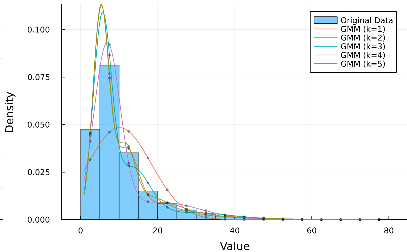
Original and GMM Modeling: Energy Demand
