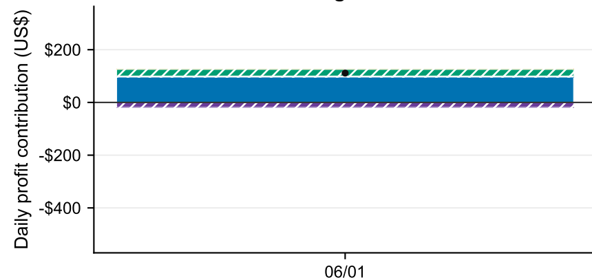
Rolling + Perfect
