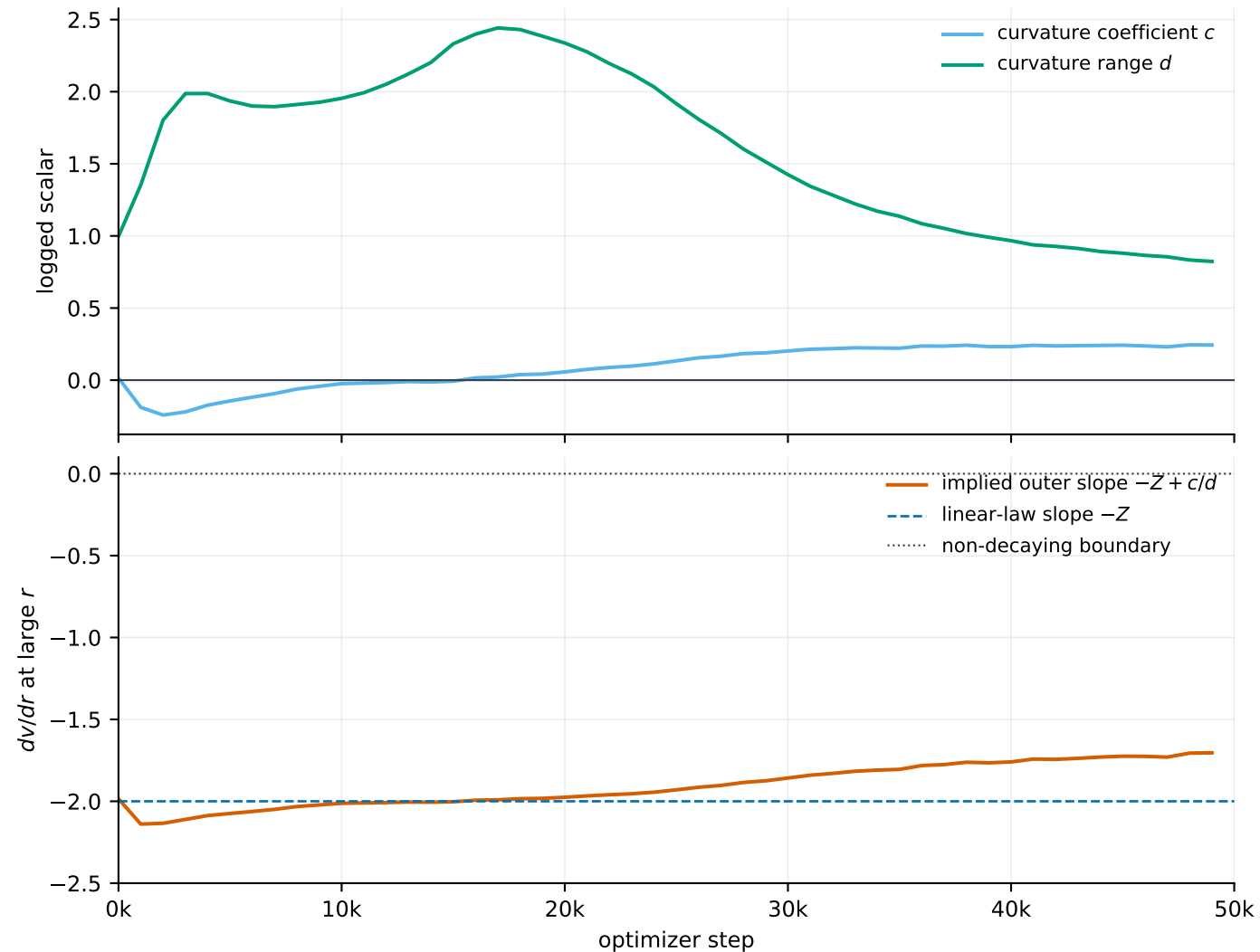
Electron-nucleus cusp law: trainable curvature and implied tail
