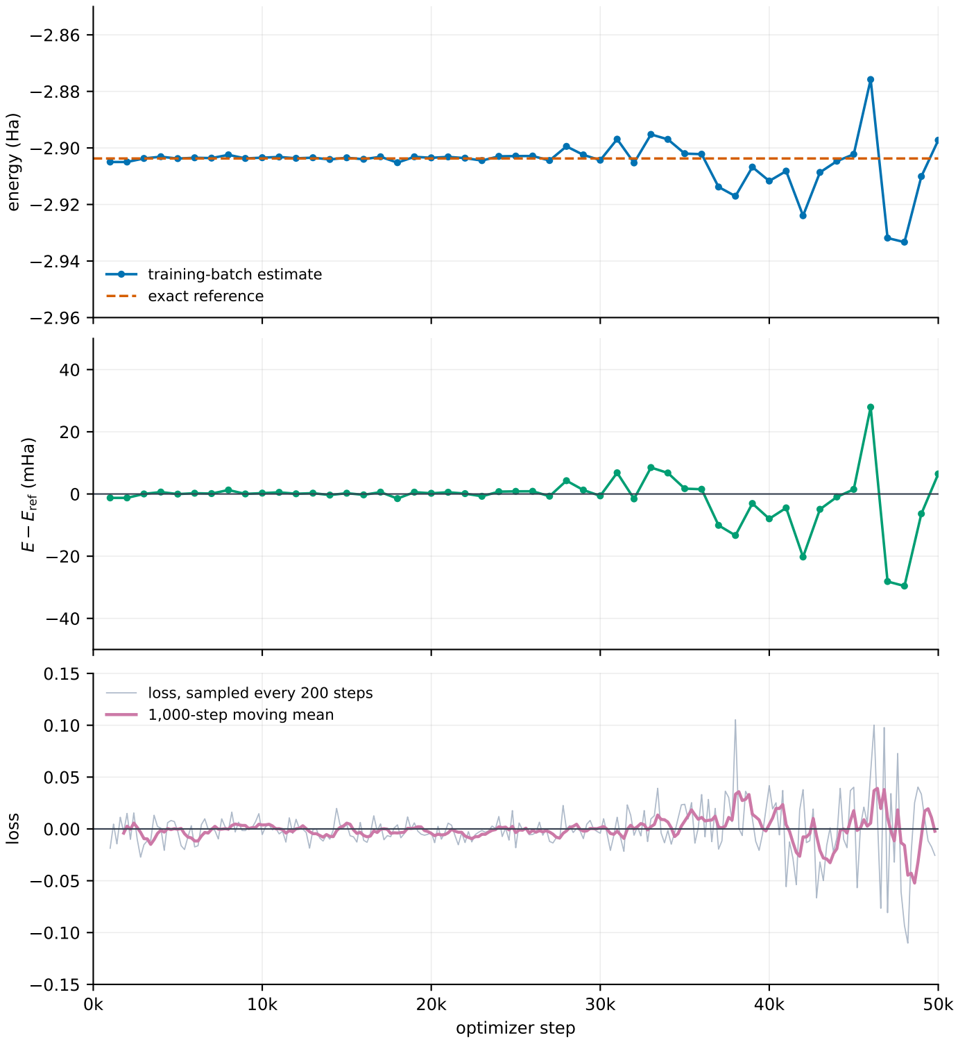
He-v1 training diagnostics — post-transient view
