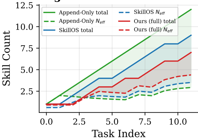
Figure 5c: Scissors Effect
