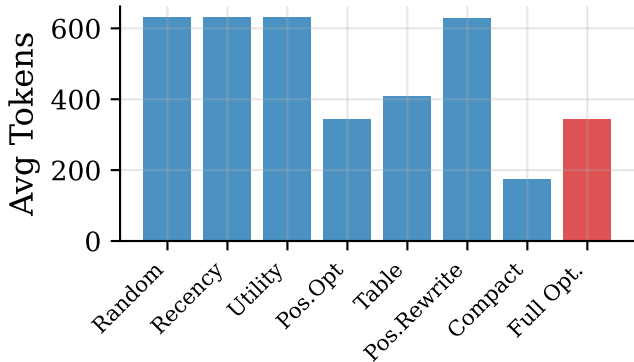
(b) Token Cost by Strategy
