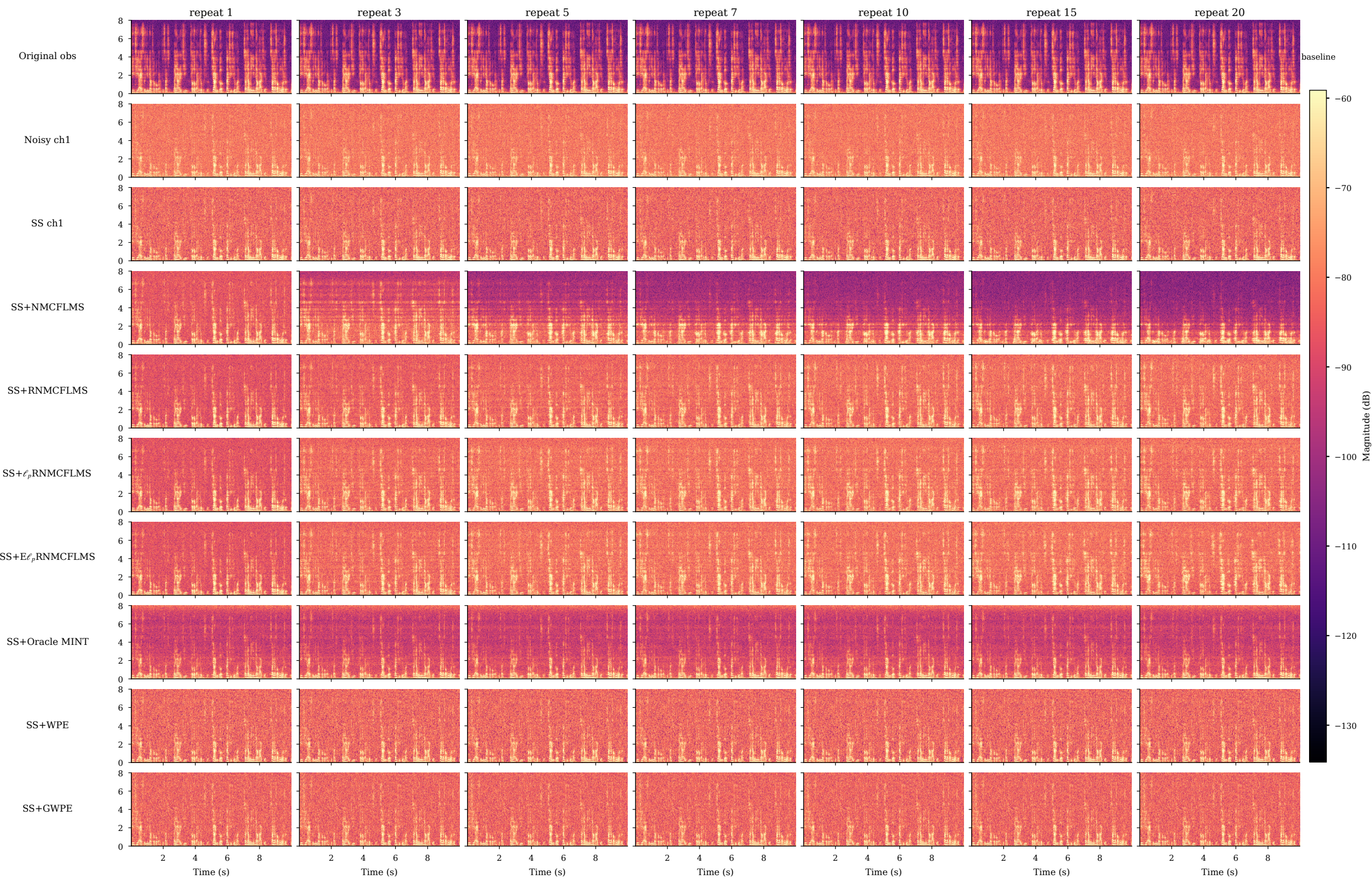
L=2048 SS-front-end spectrogram — TIMIT sample 7, reg=0.1, SNR 5 dB
