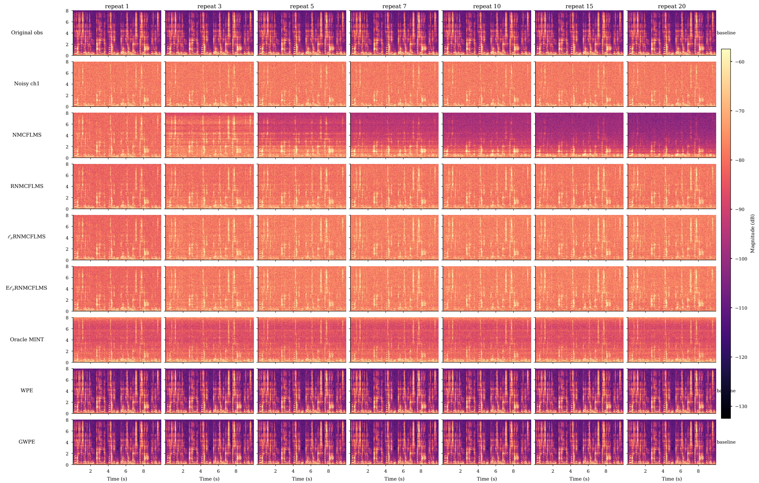
L=2048 No-SS spectrogram – TIMIT sample 5, reg=0.05, SNR 5 dB
