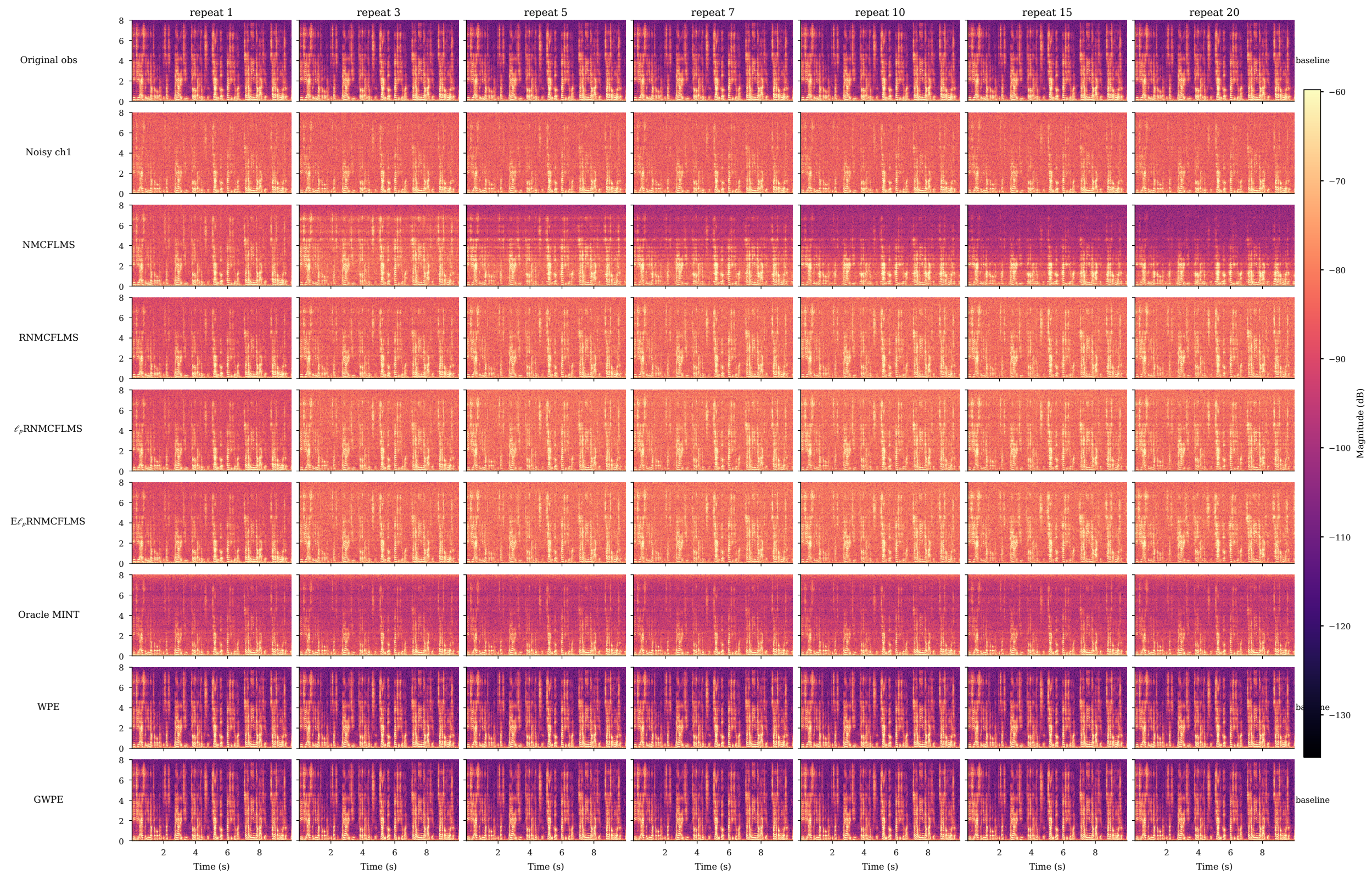
L=2048 No-SS spectrogram — TIMIT sample 7, reg=0.05, SNR 10 dB
