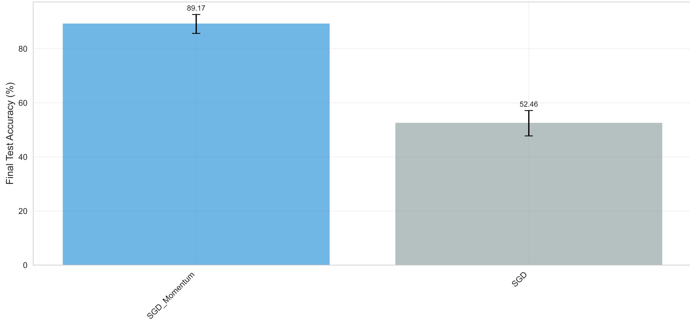
Momentum Effect: Ablation Study Results
