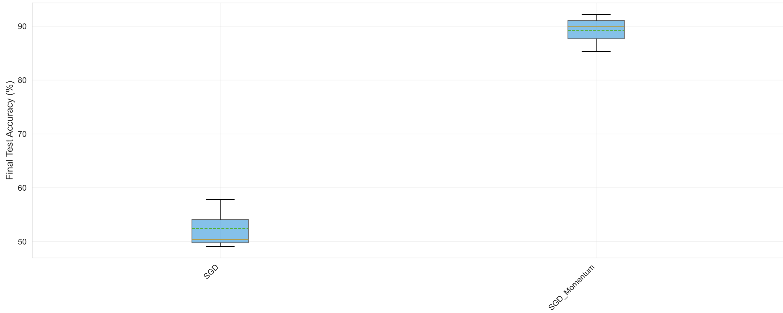
Momentum Effect: Distribution Across Seeds
