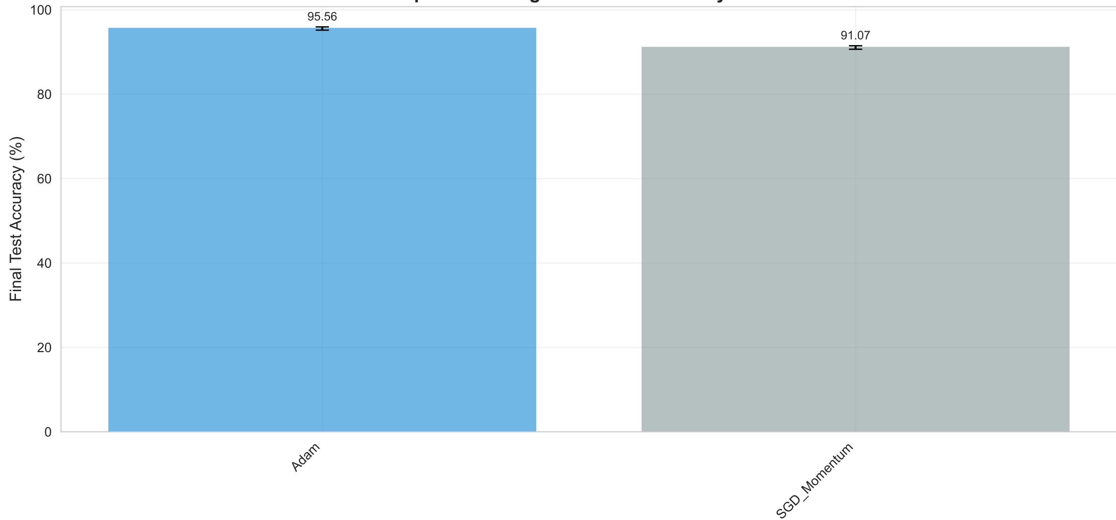
Adaptive Learning Rate: Ablation Study Results
