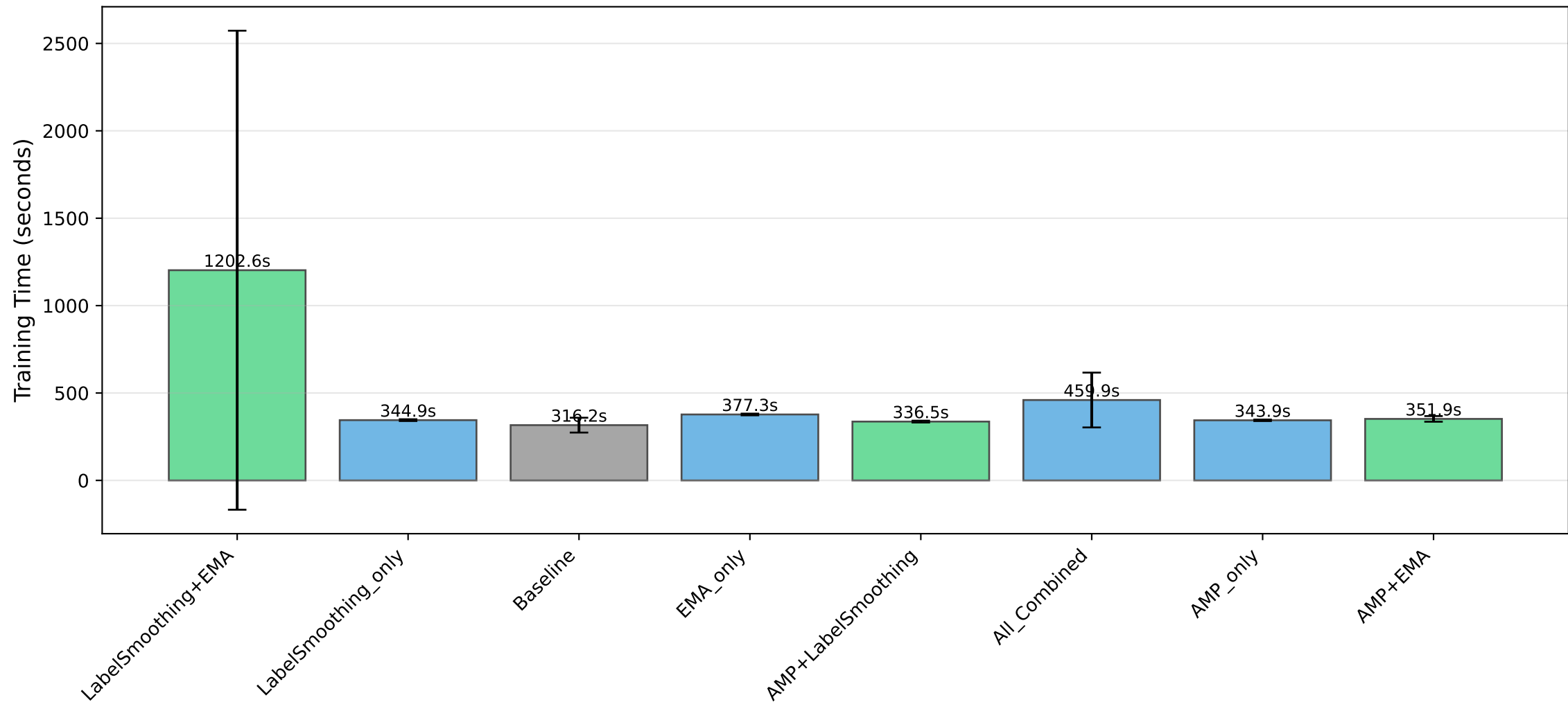
Training Time Comparison (Lower is better)
