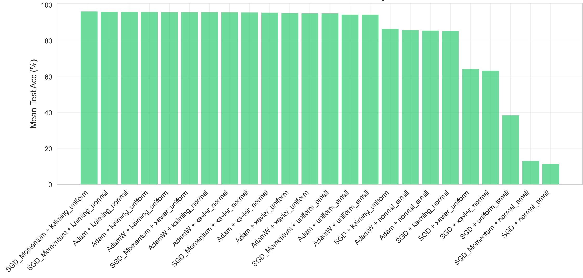
Initialization Ablation: Ablation Study Results
