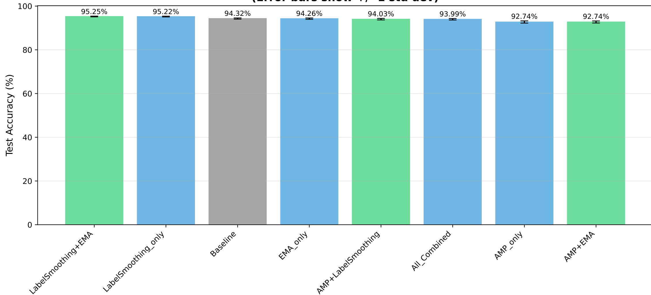
Advanced Training Features: Ablation Study Results (Error bars show +/- 1 std dev)
