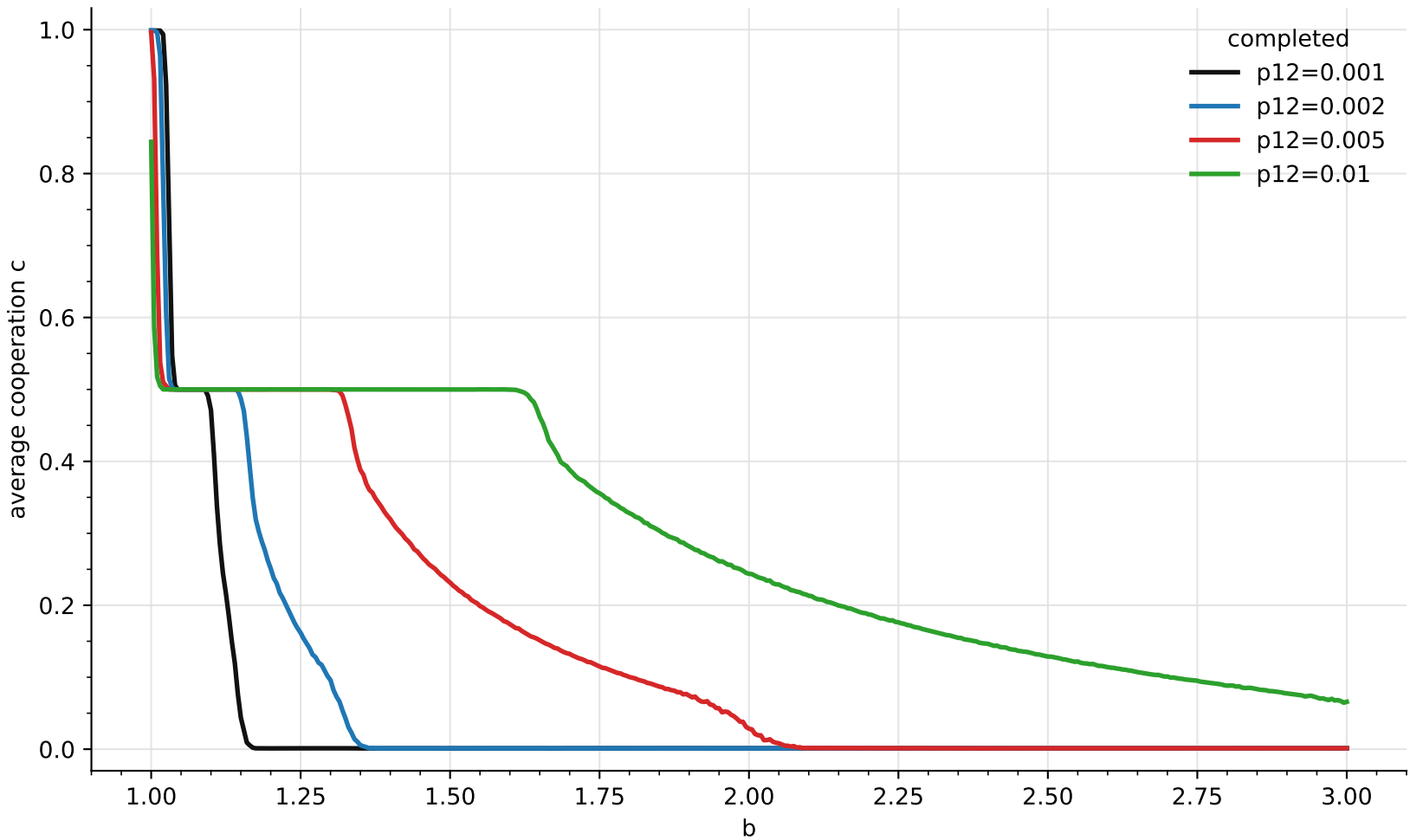
Fig. 3 Fermi beta=5 partial (4 completed curves)
