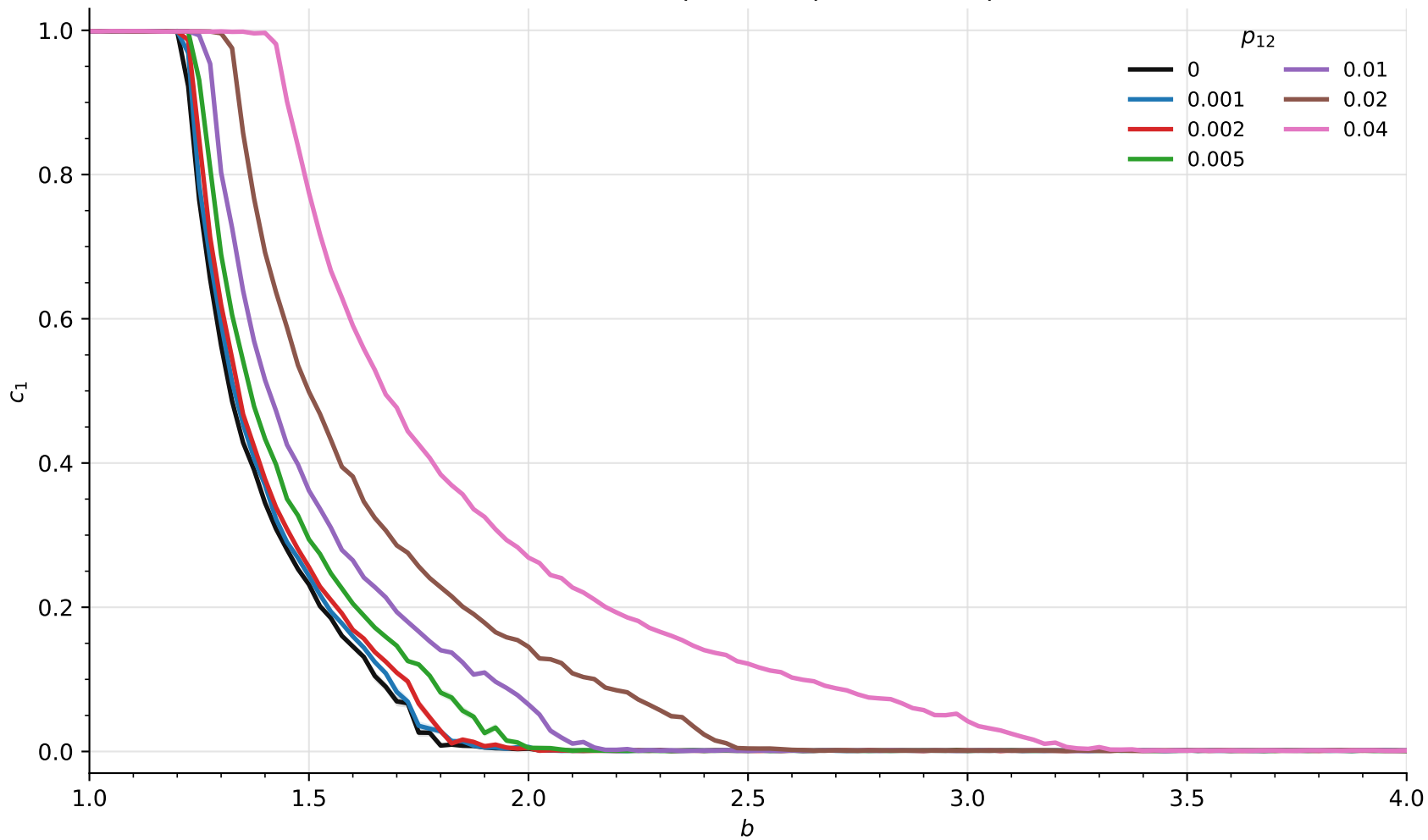
Fig. 4 degree-weighted linear update N1=1000, N2=100, reps=30, alpha=1, clamp=[1/3,3]
