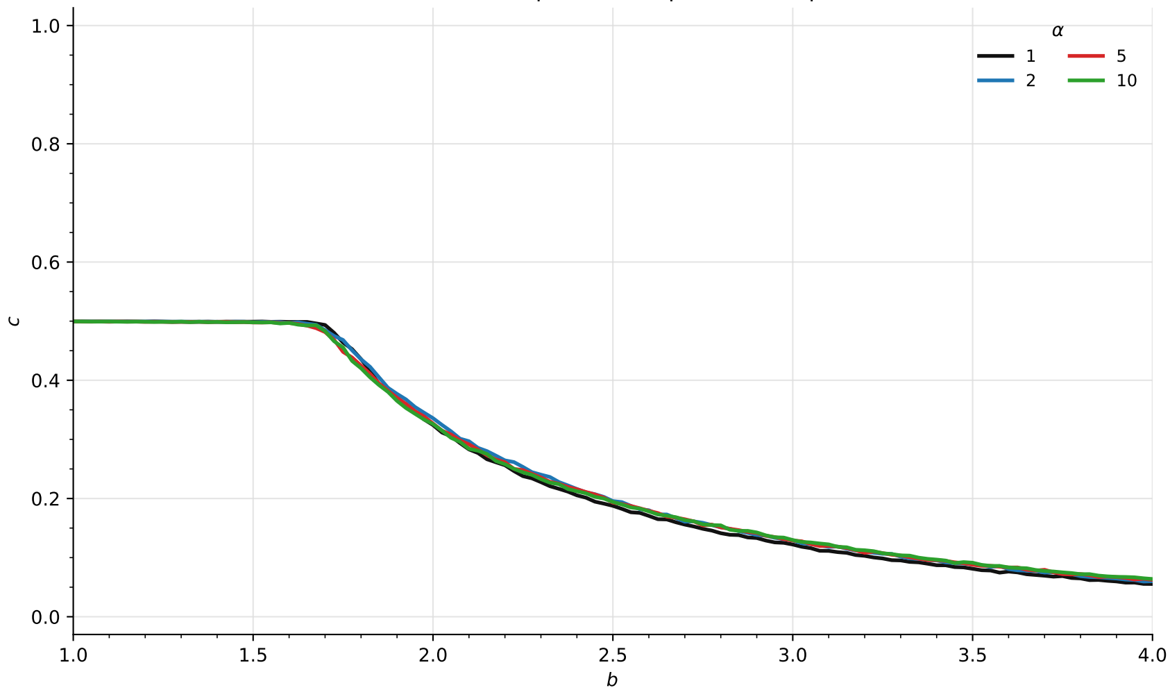
Global cooperation: alpha sweep N1=1000, N2=100, p12=0.1, reps=30, clamp=[1/3,3]
