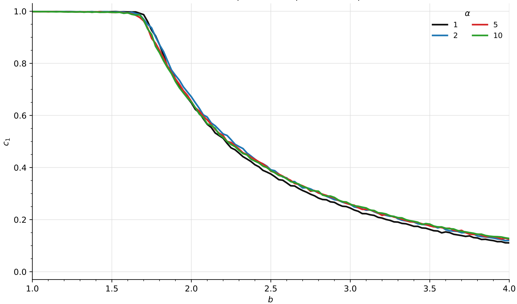
Degree-weighted linear update: alpha sweep N1=1000, N2=100, p12=0.1, reps=30, clamp=[1/3,3]
