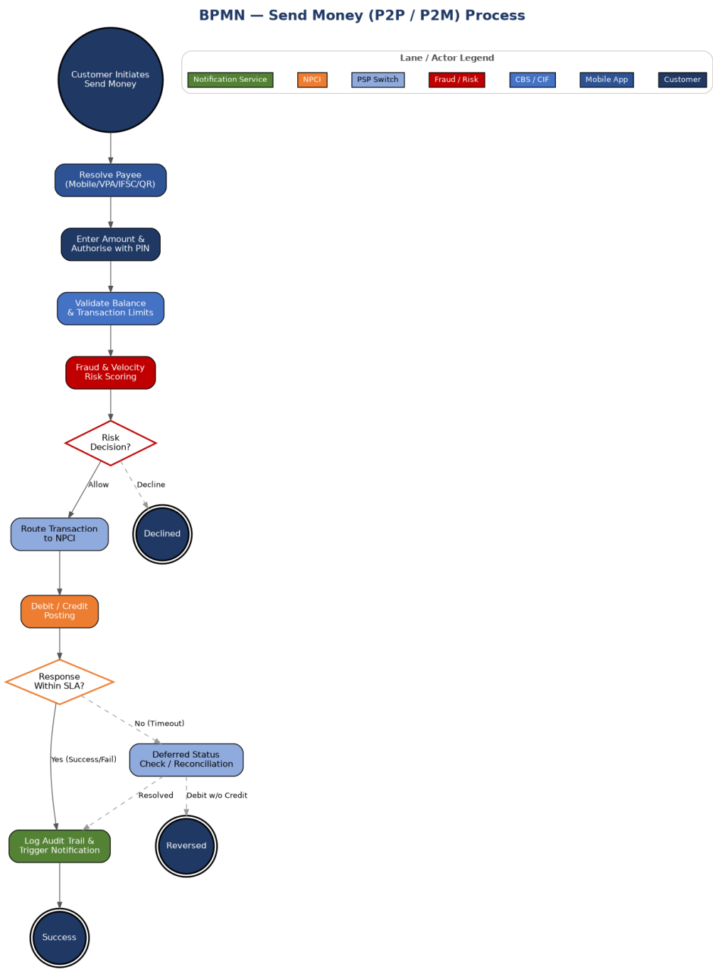
Figure 4 — BPMN: Send Money (P2P / P2M) Process
