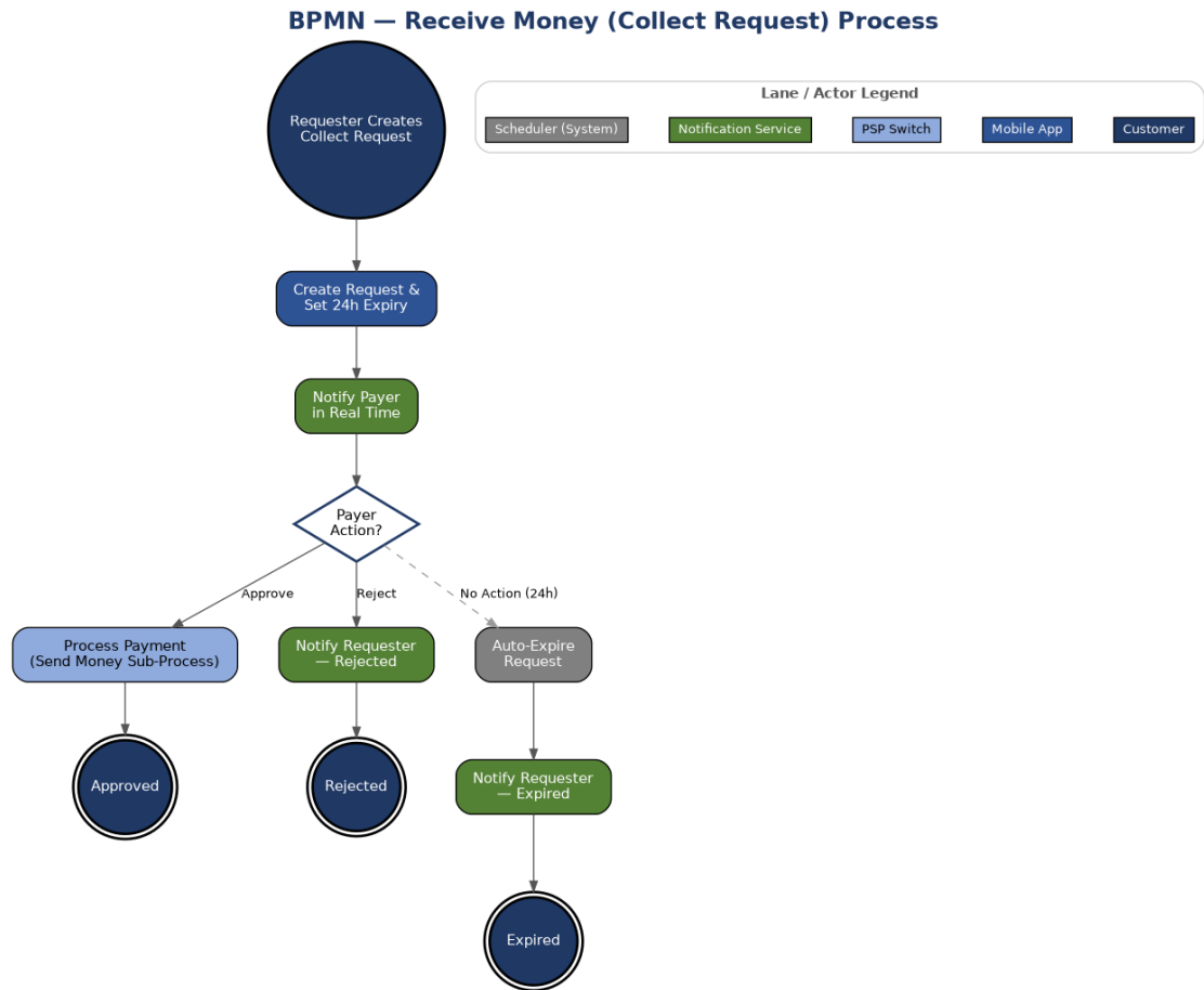
Figure 5 — BPMN: Receive Money (Collect Request) Process
