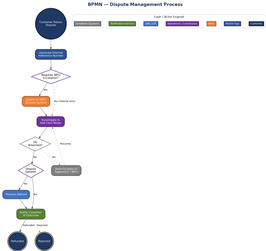
Figure 6 — BPMN: Dispute Management Process
