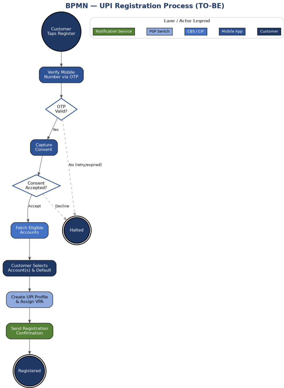
Figure 1 — BPMN: UPI Registration Process (TO-BE)
