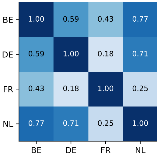
(a) Residual correlations
