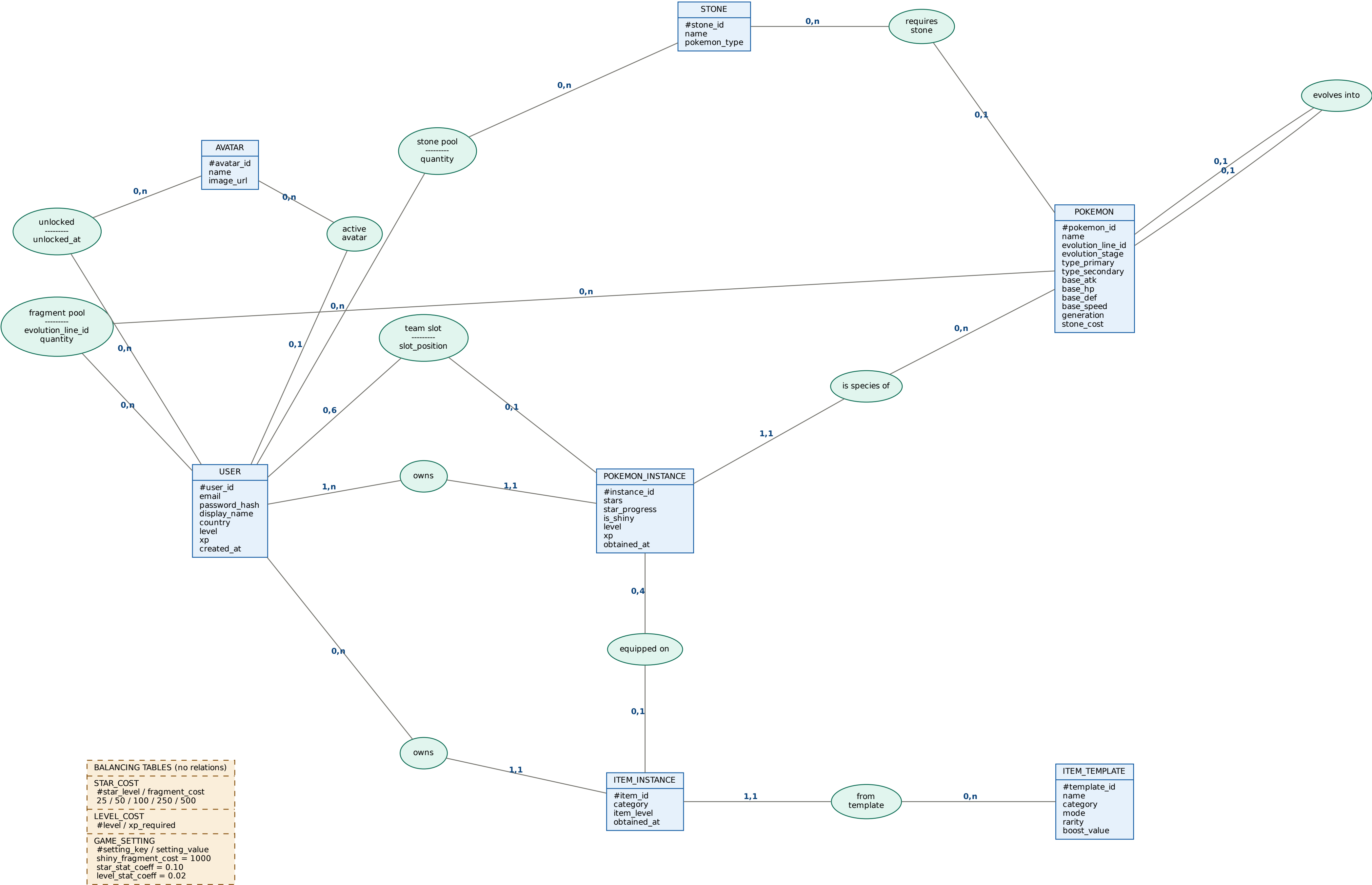
Conceptual Data Model (Merise) - Pokemon Web Game
