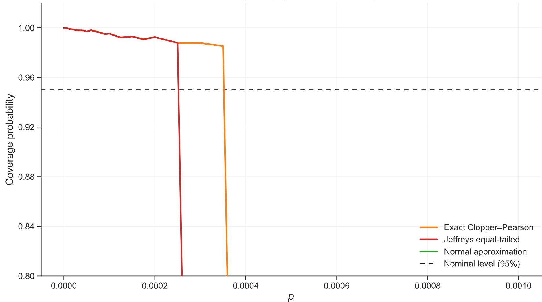
Coverage vs p ( n=10000 , \rho=0.1 )
