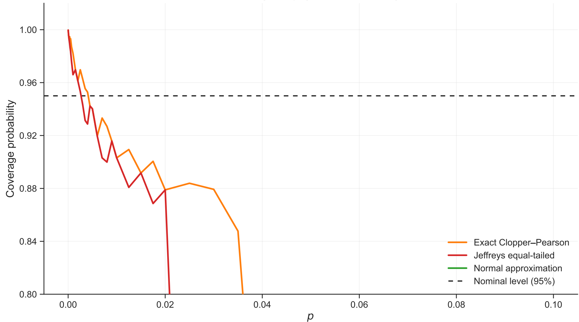
Coverage vs p (n=100, rho=0.05)
