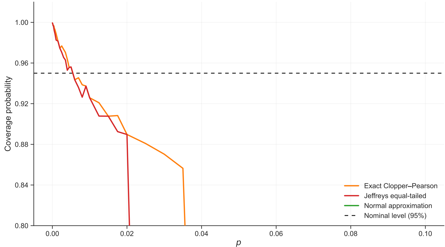
Coverage vs p ( n=100 , \rho=0.15 )
