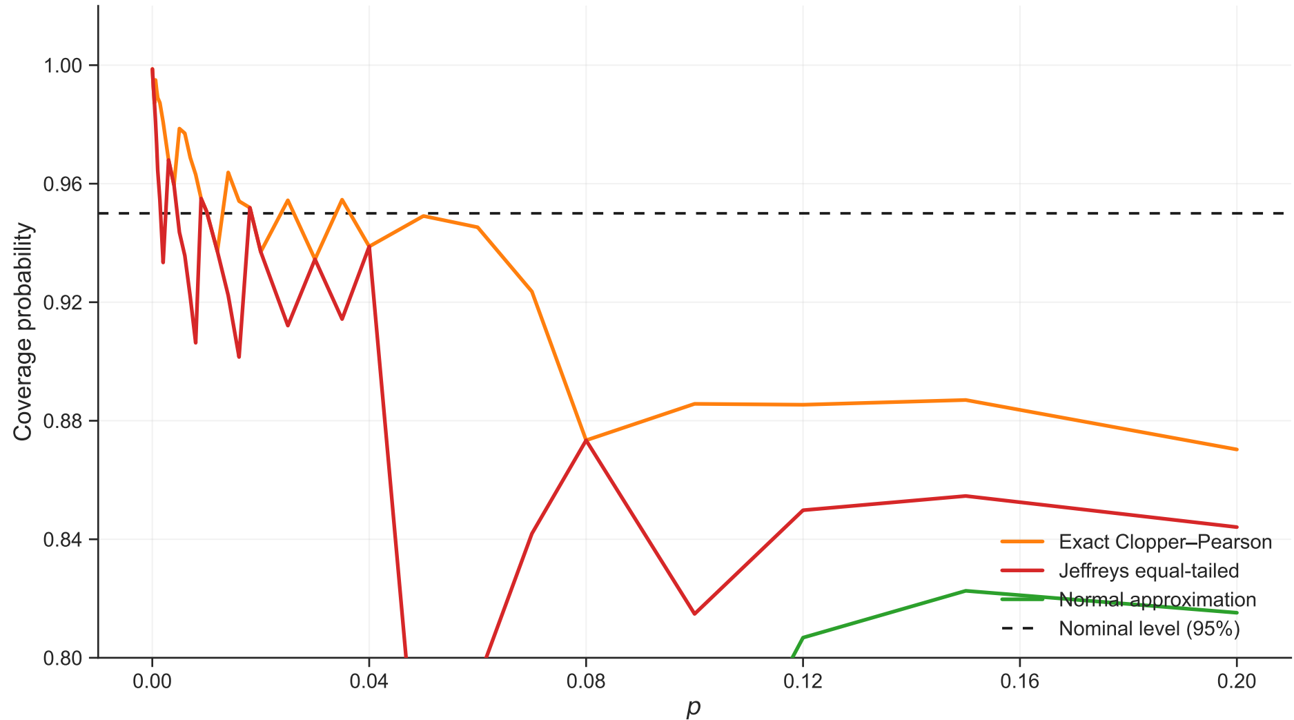
Coverage vs p ( n=50 , \rho=0.02 )
