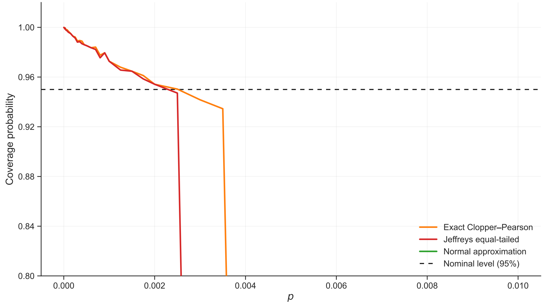
Coverage vs p (n=1000, rho=0.1)
