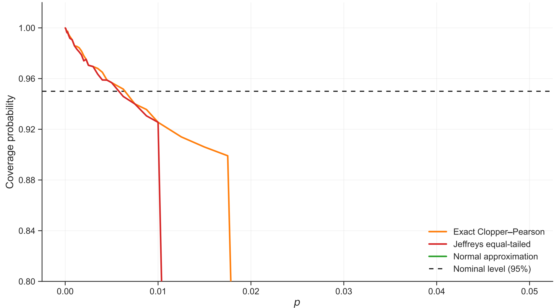
Coverage vs p (n=200, rho=0.2)
