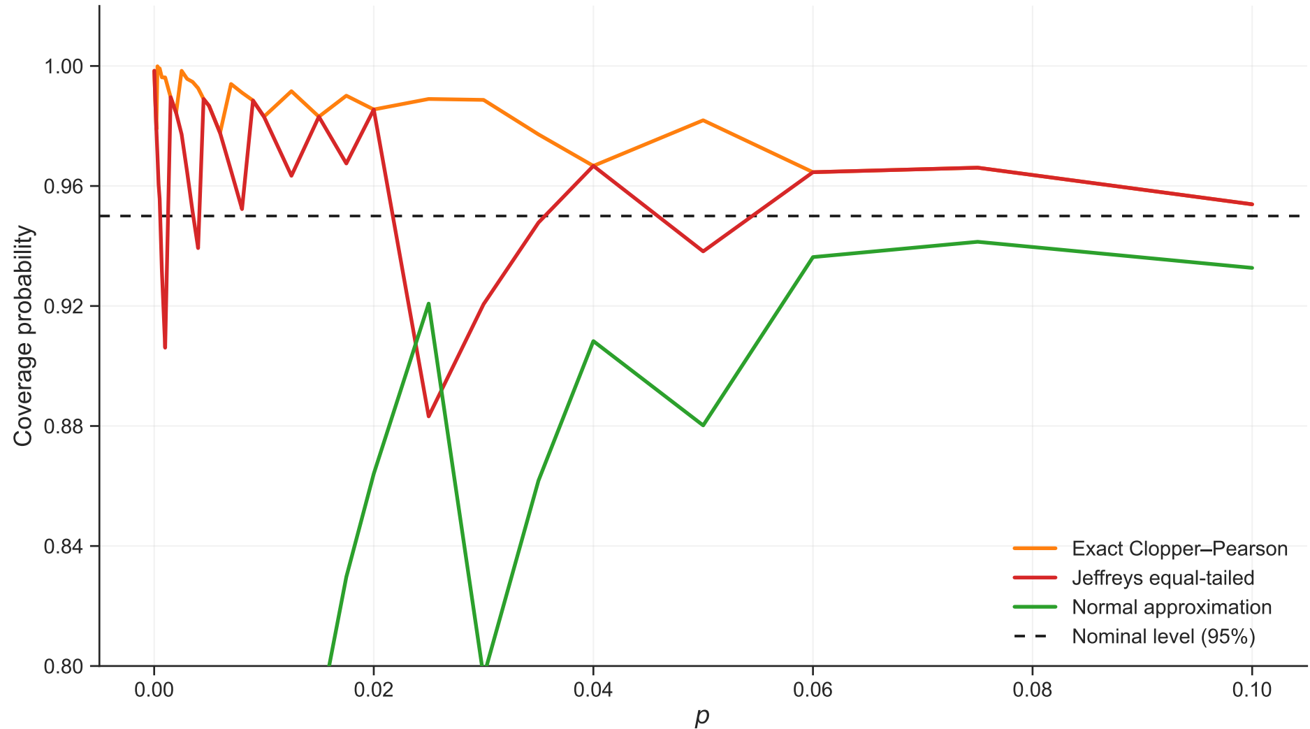
Coverage vs p ( n=100 , \rho=0.0 )
