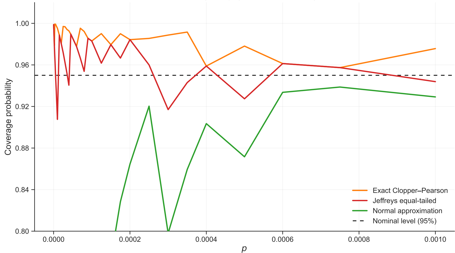
Coverage vs p ( n=10000 , \rho=0.0 )
