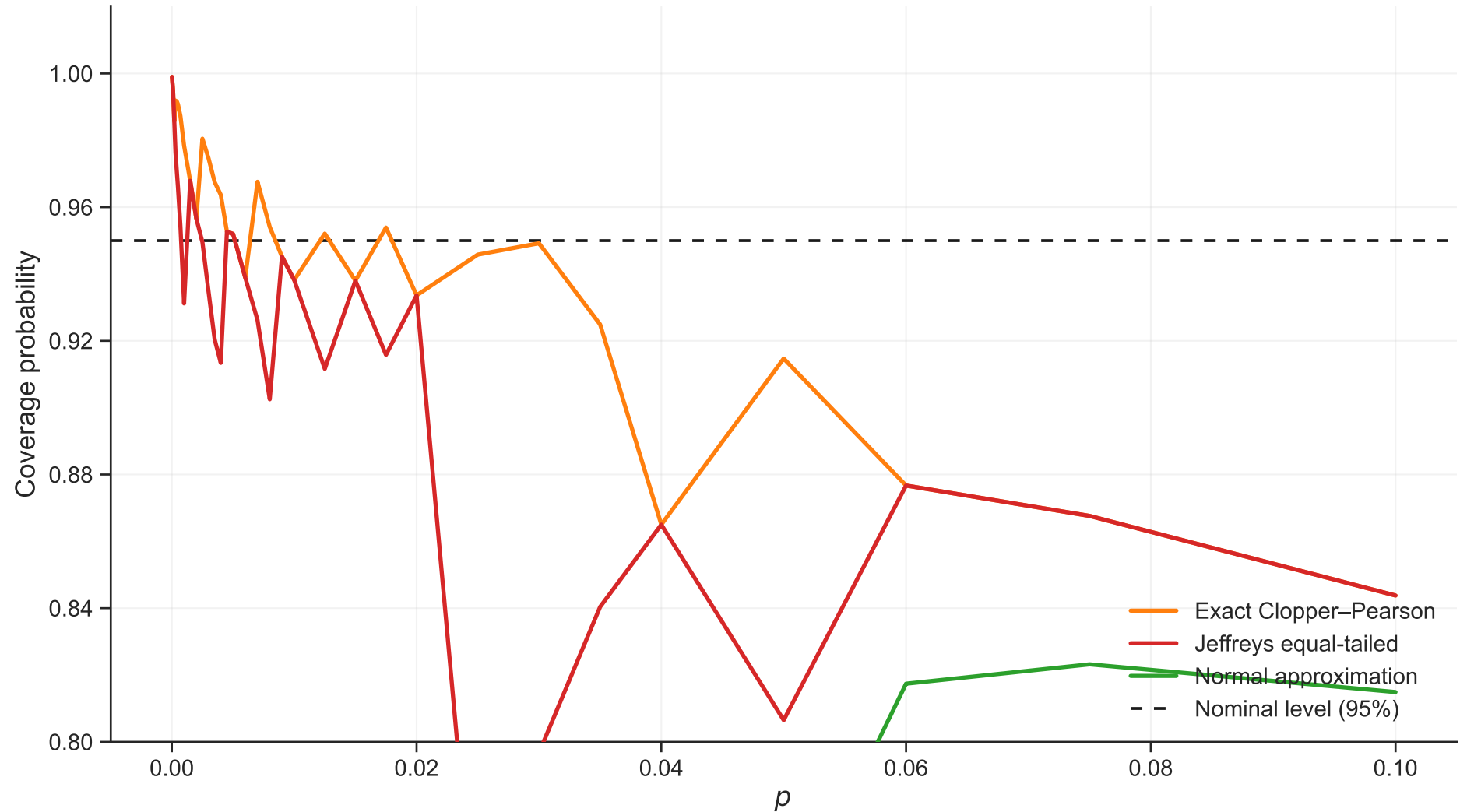
Coverage vs p ( n=100 , \rho=0.01 )
