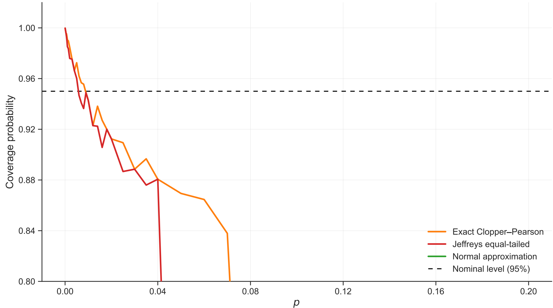
Coverage vs p ( n=50 , \rho=0.15 )
