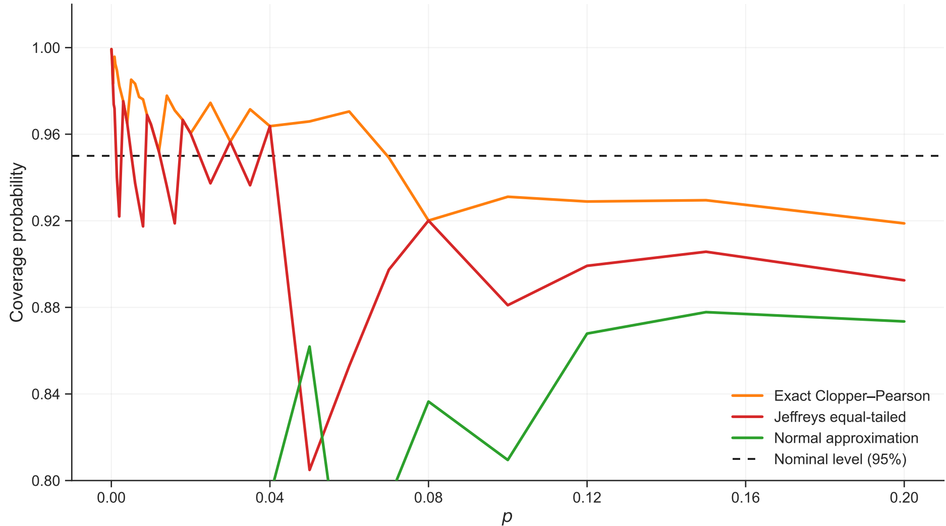
Coverage vs p (n=50, rho=0.01)
