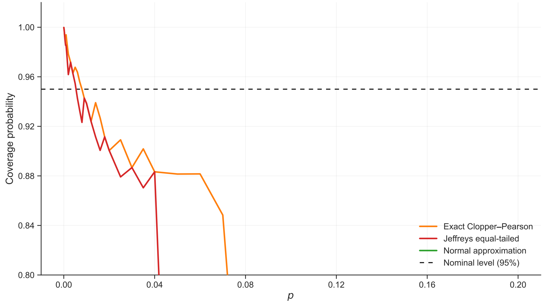
Coverage vs p ( n=50 , \rho=0.1 )
