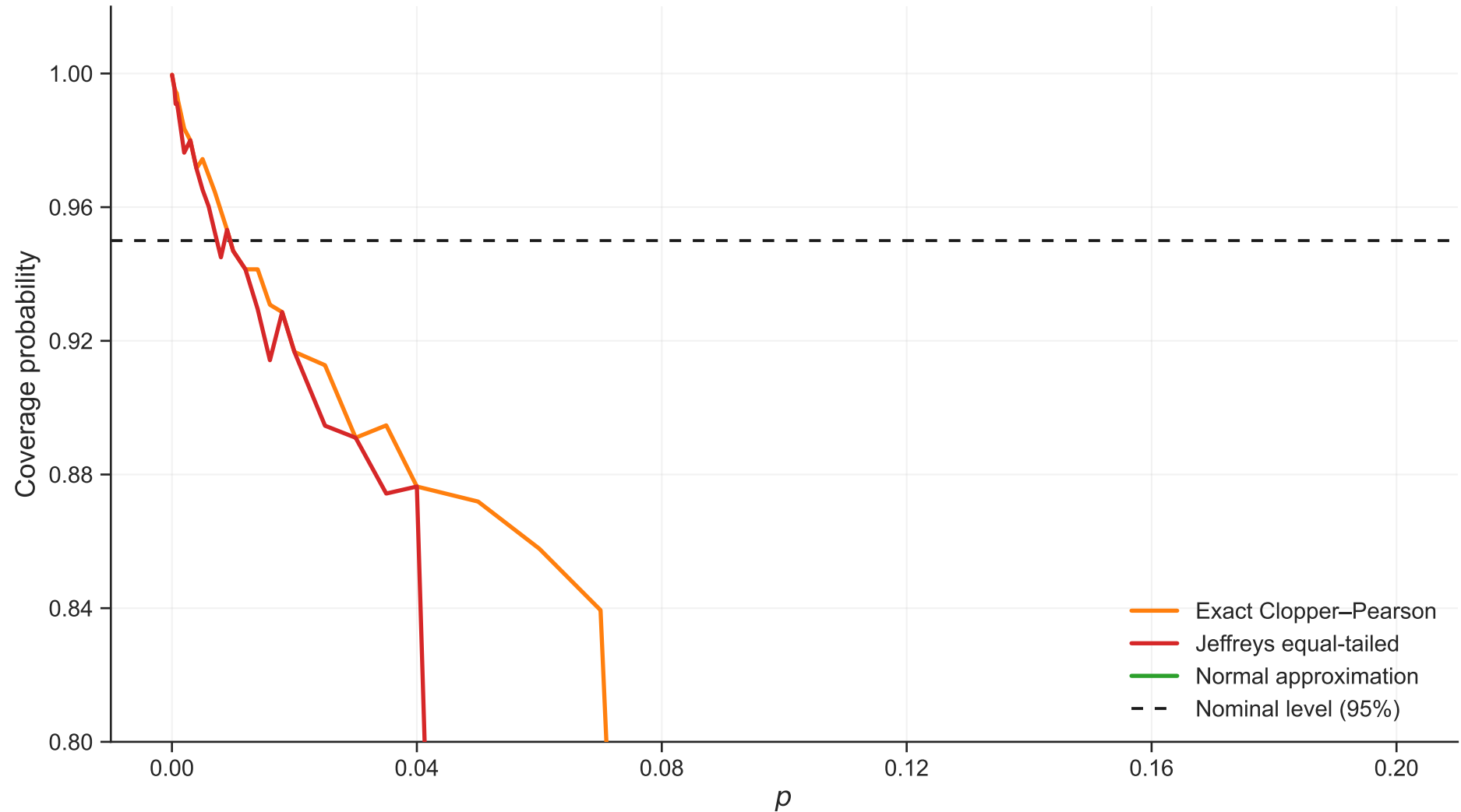
Coverage vs p ( n=50 , \rho=0.2 )
