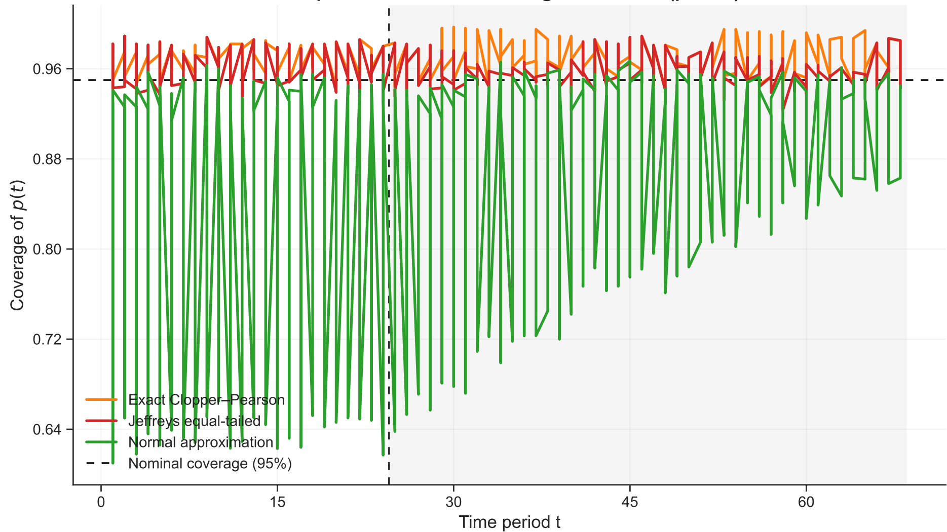
Temporal evolution of coverage under drift ( \hat{p}=0.01 )
