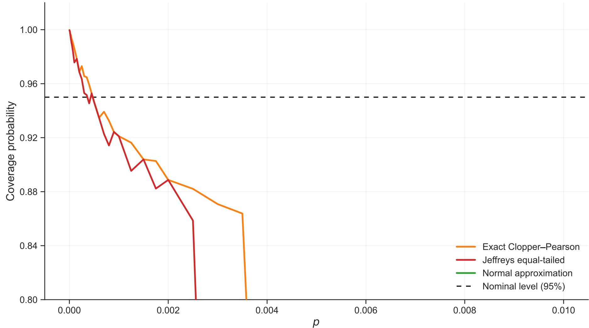
Coverage vs p ( n=1000 , \rho=0.01 )
