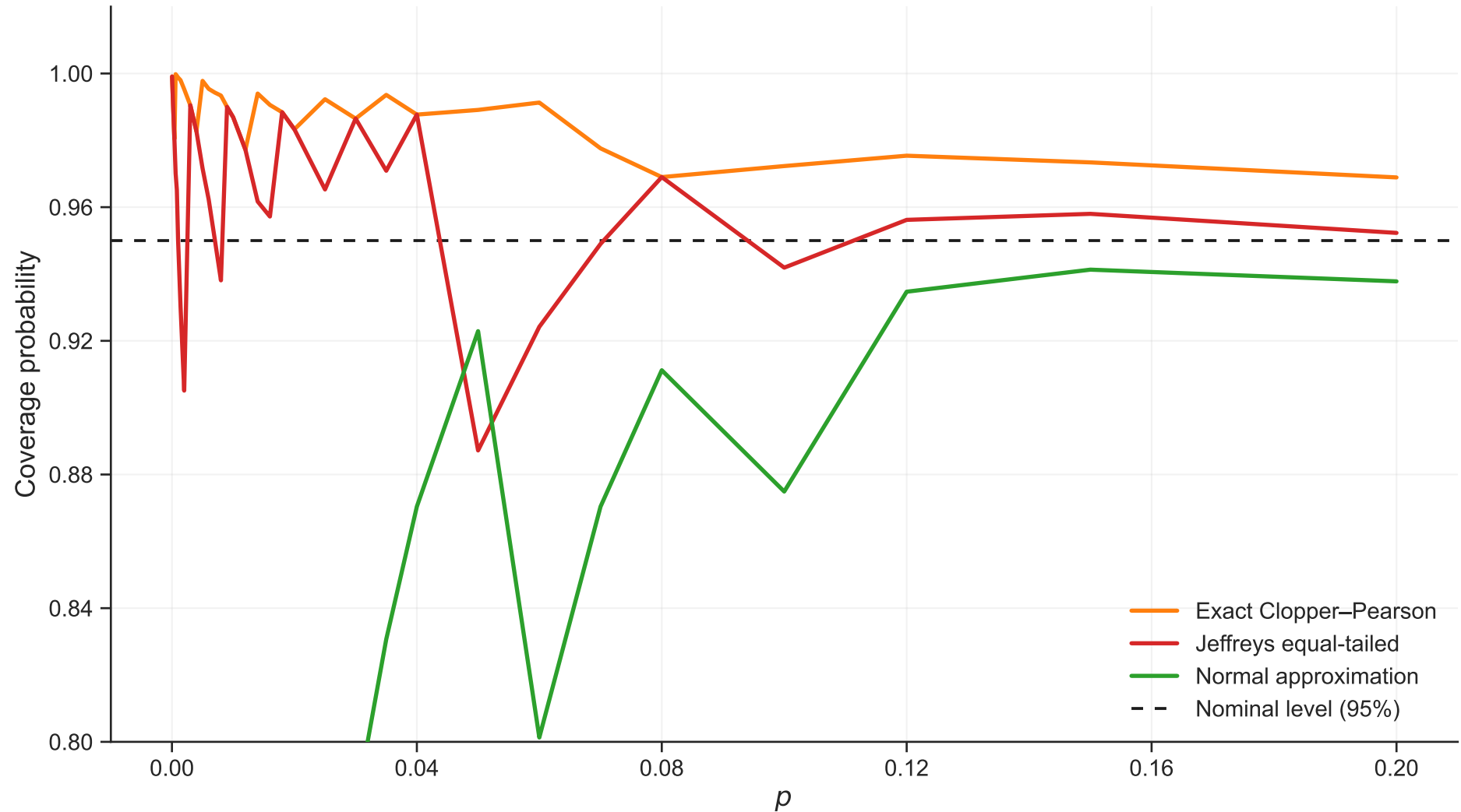
Coverage vs p ( n=50 , \rho=0.0 )
