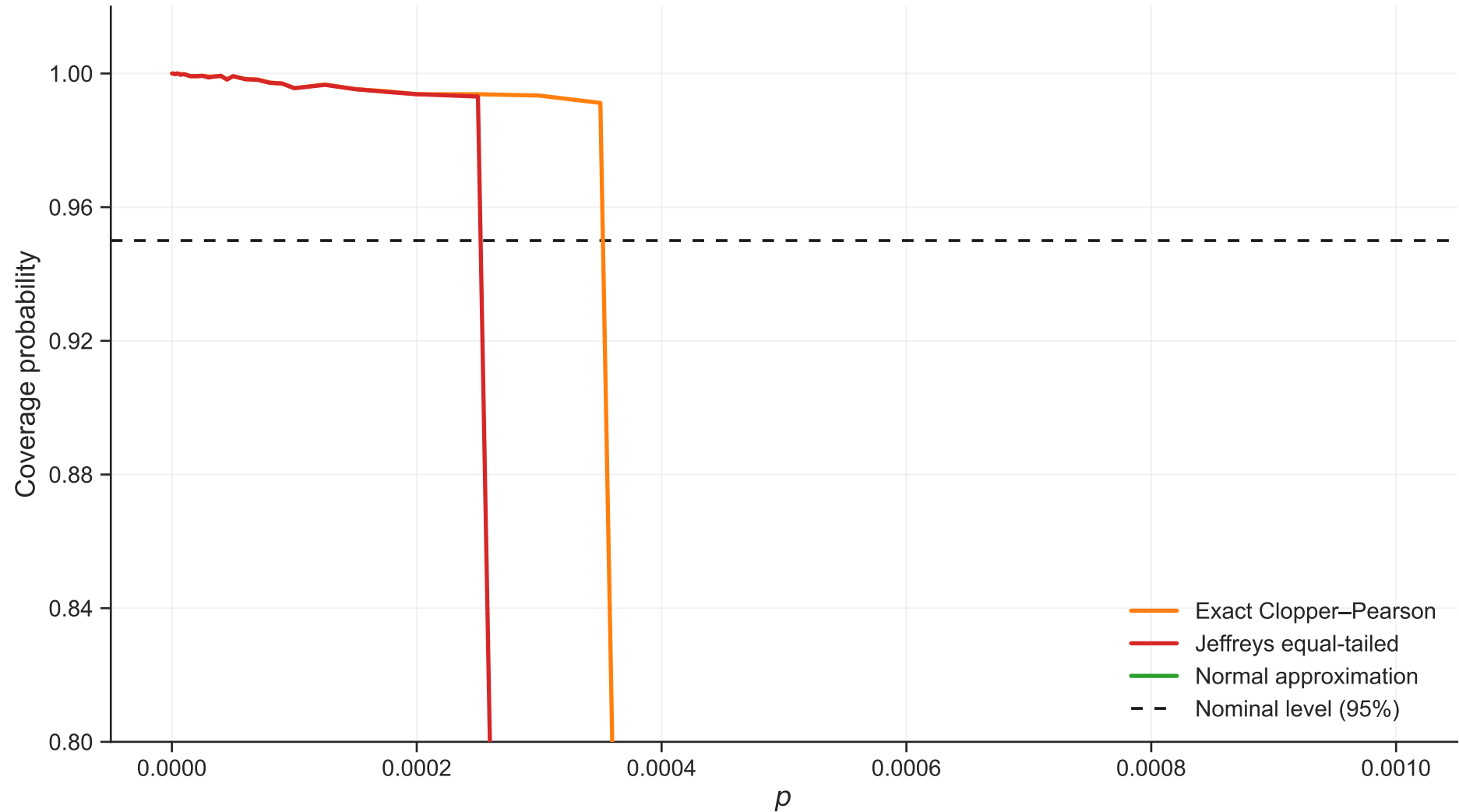
Coverage vs p (n=10000, rho=0.15)
