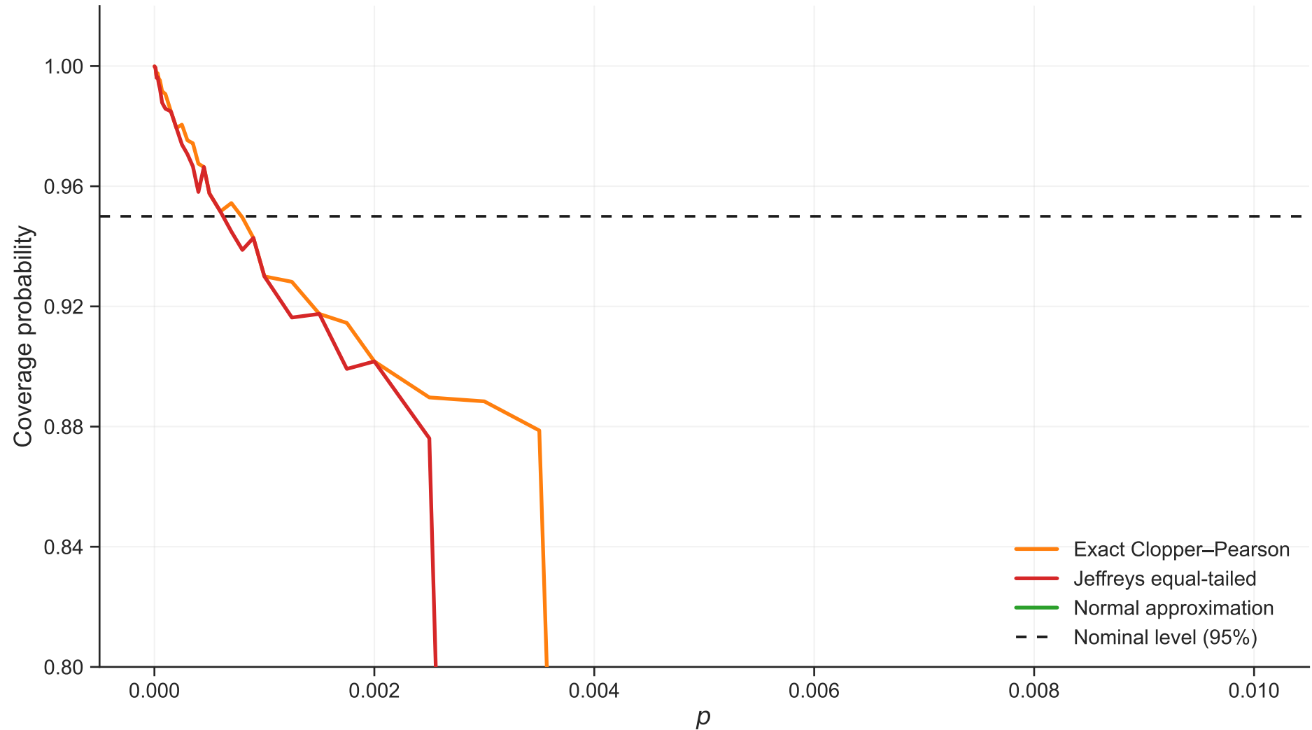
Coverage vs p ( n=1000 , \rho=0.02 )
