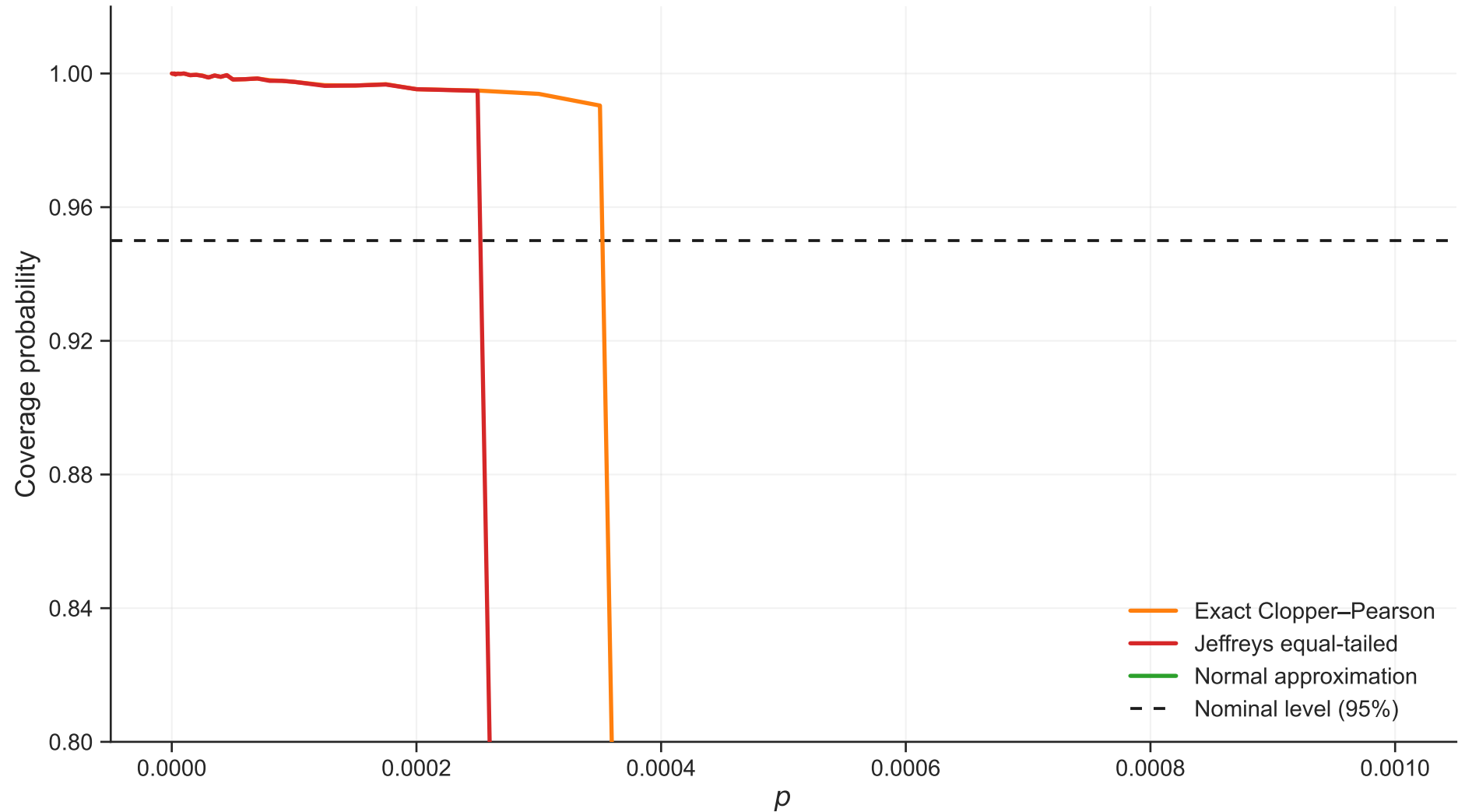
Coverage vs p ( n=10000 , \rho=0.2 )
