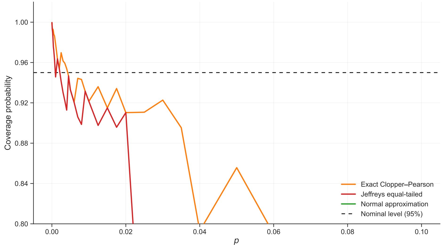
Coverage vs p (n=100, rho=0.02)
