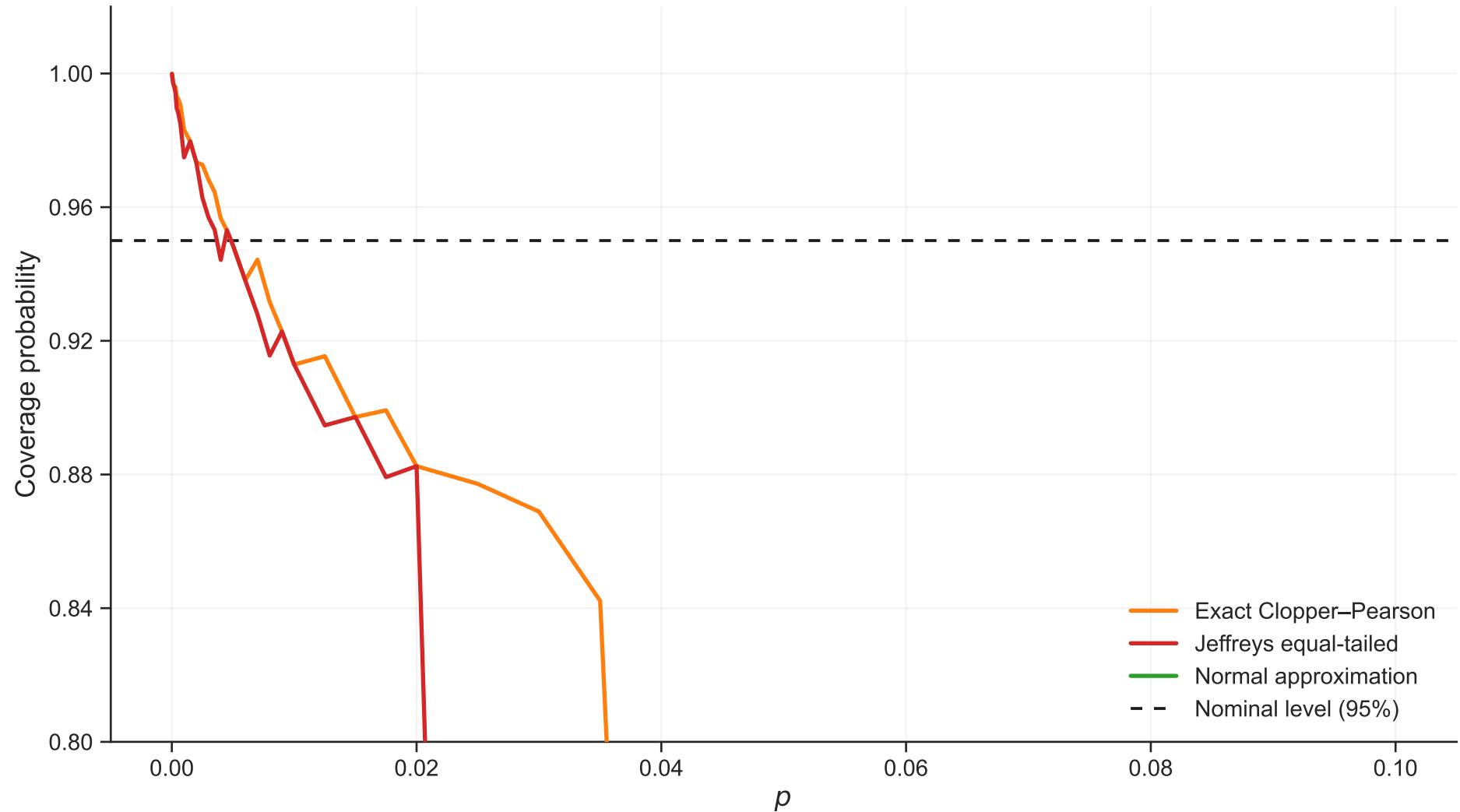
Coverage vs p (n=100, rho=0.1)
