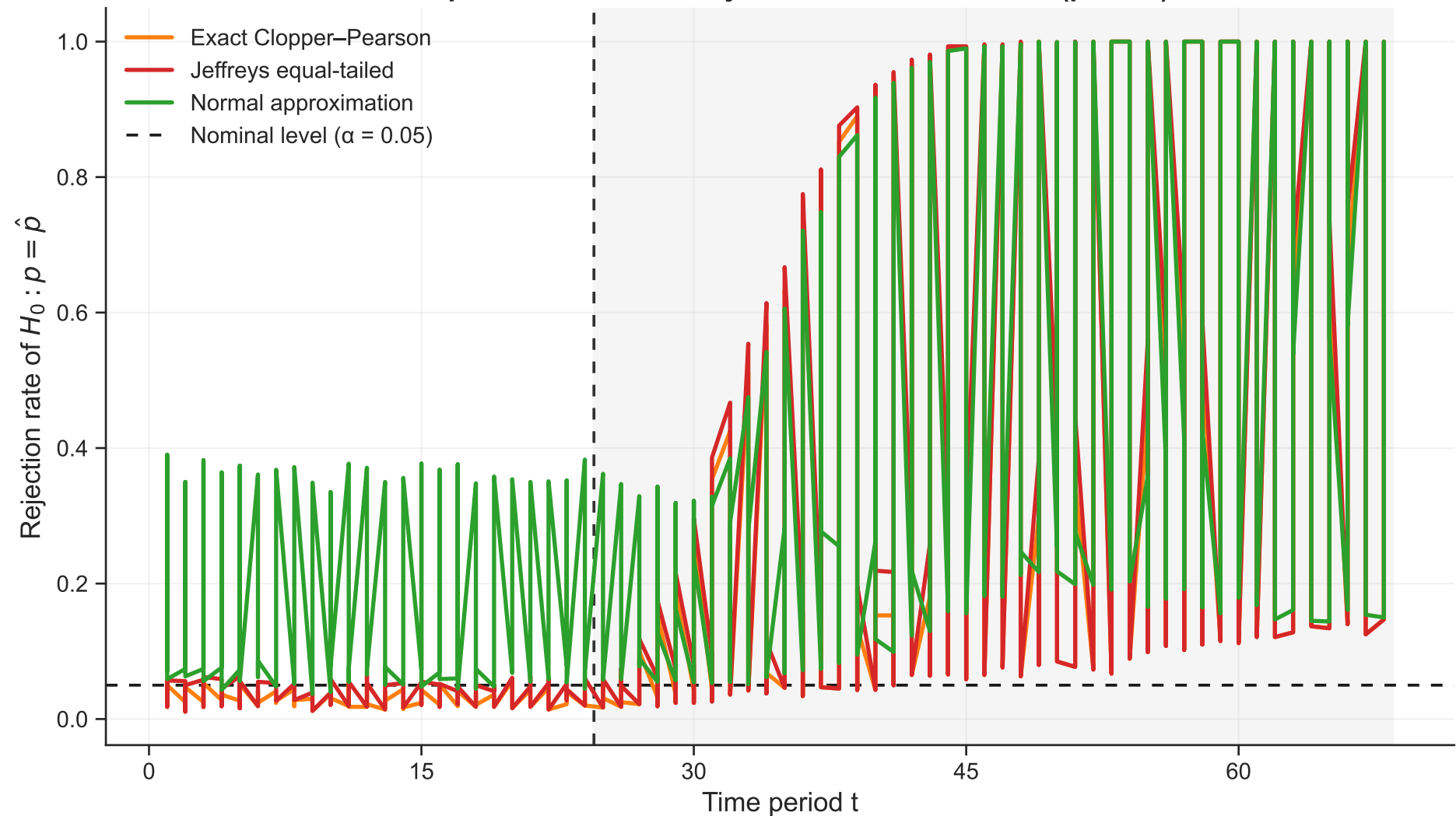
Temporal evolution of rejection rates under drift ( \hat{p}=0.01 )
