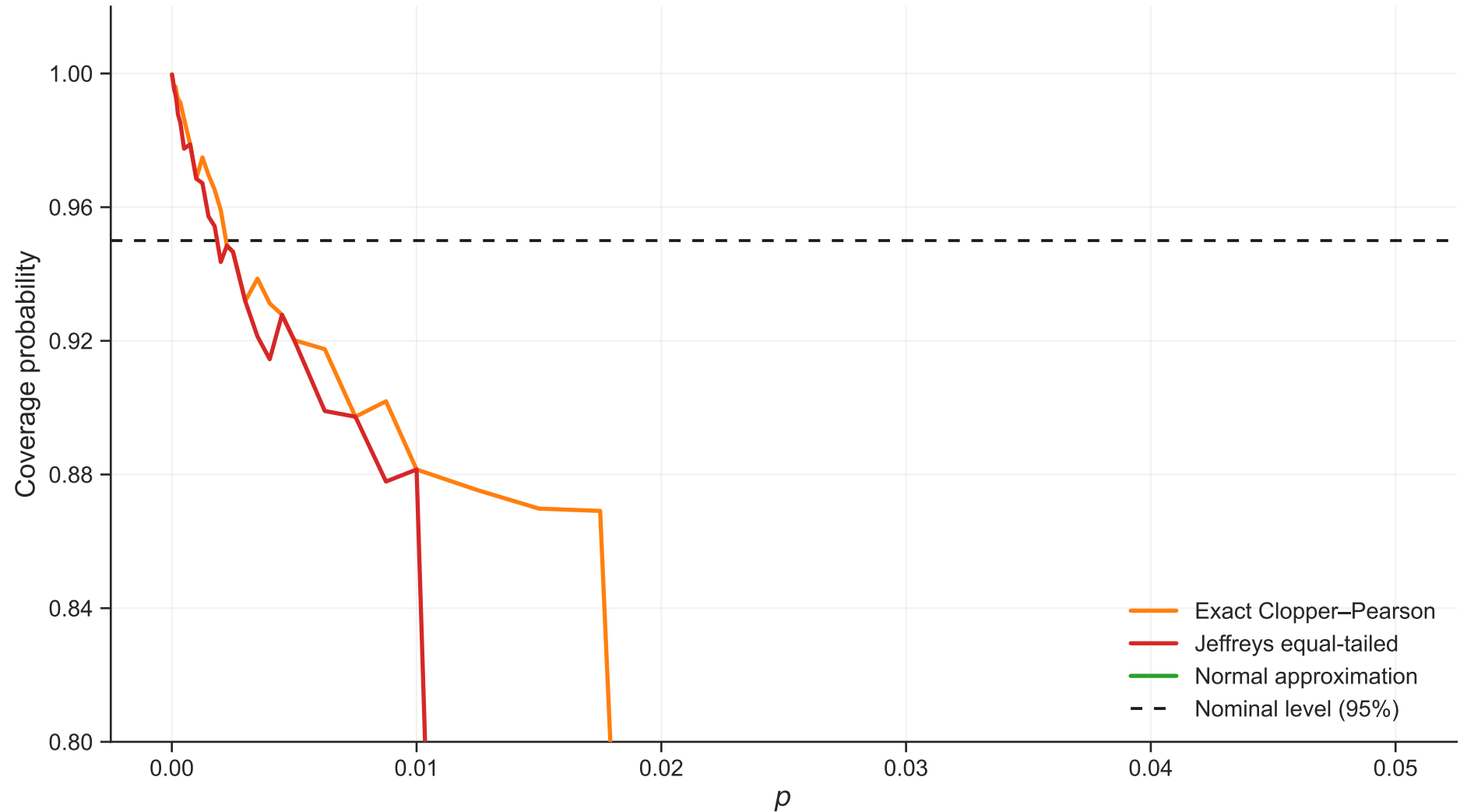
Coverage vs p (n=200, rho=0.05)
