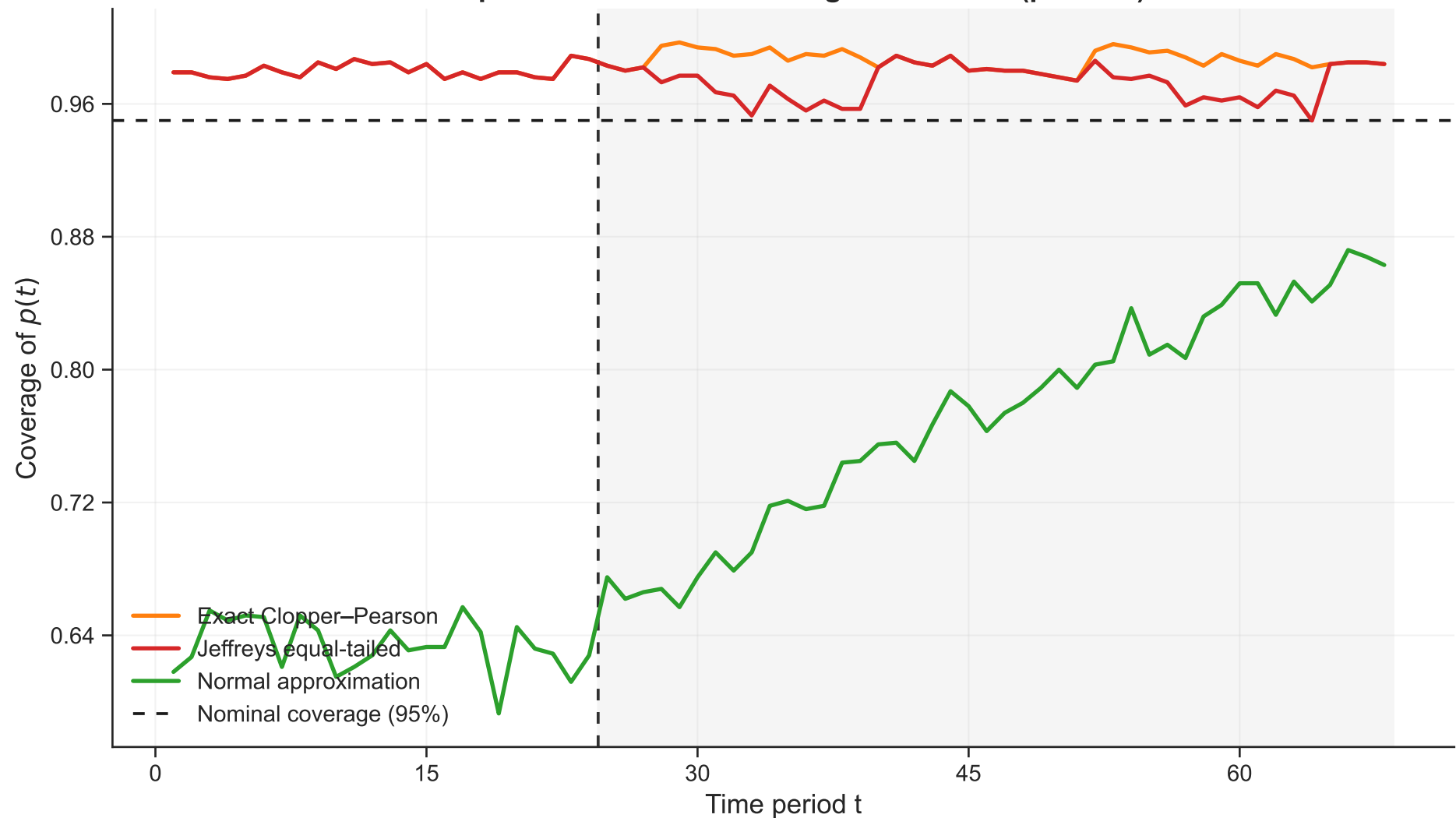
Temporal evolution of coverage under drift ( \hat{p}=0.001 )
