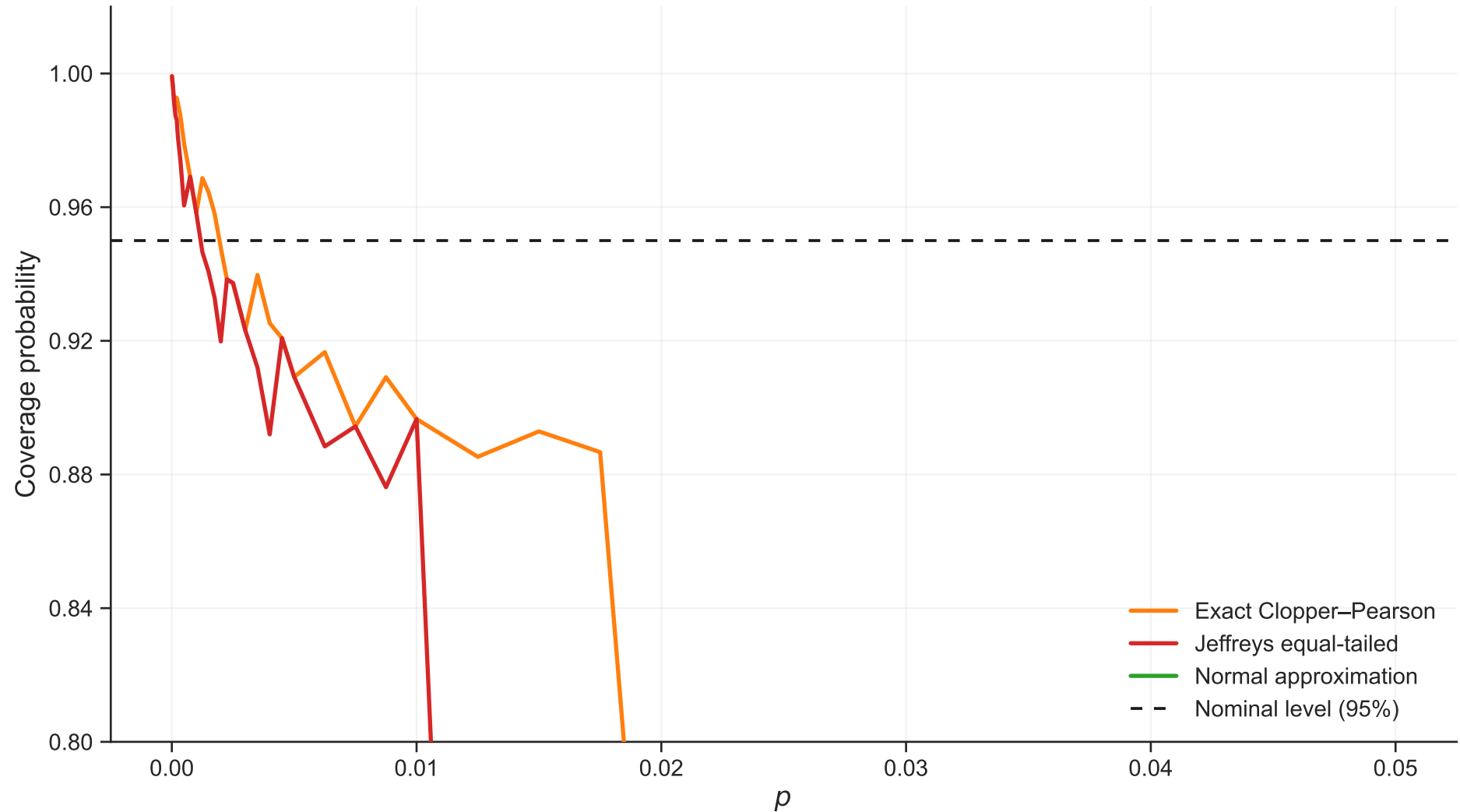
Coverage vs p (n=200, rho=0.02)
