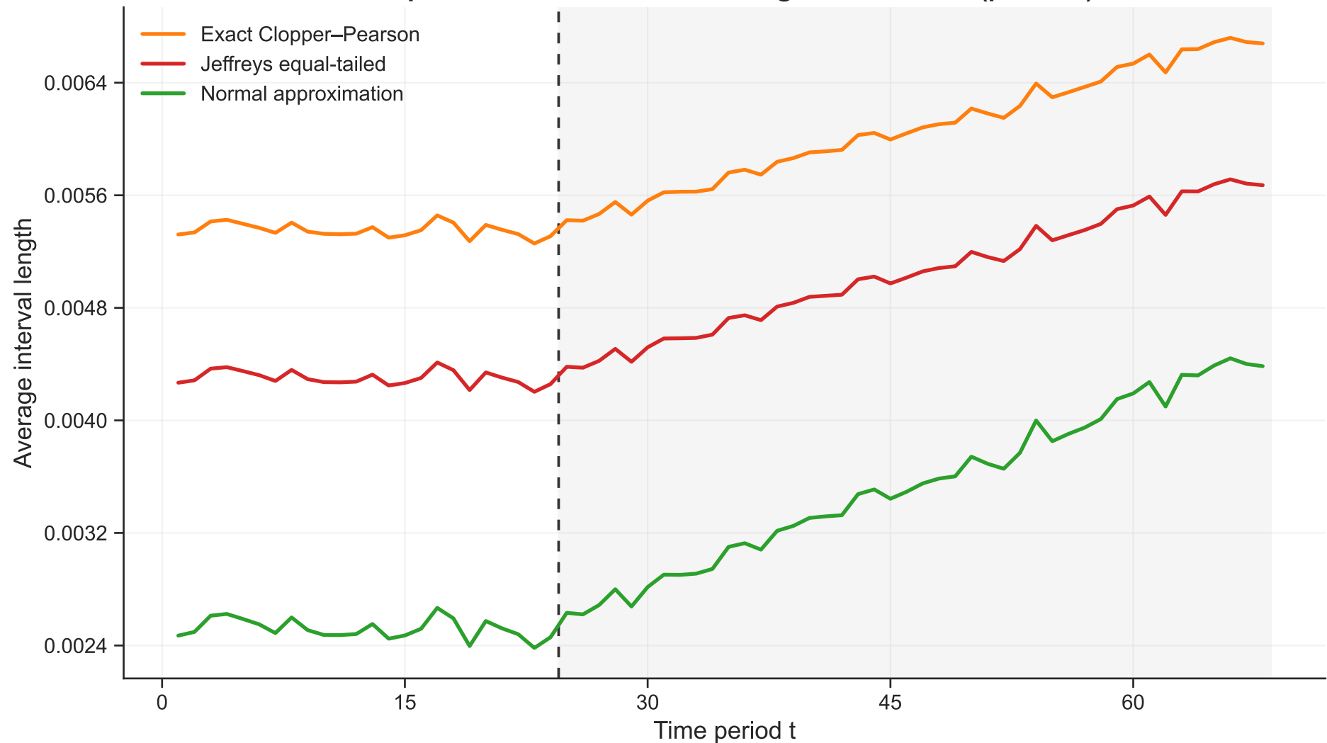
Temporal evolution of interval lengths under drift ( \hat{p}=0.001 )
