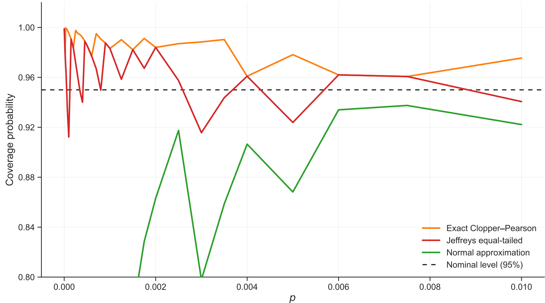
Coverage vs p ( n=1000 , \rho=0.0 )
