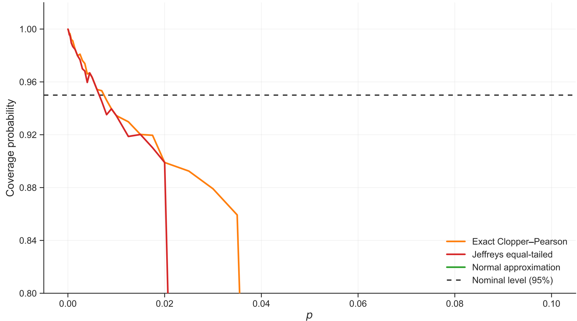
Coverage vs p ( n=100 , \rho=0.2 )
