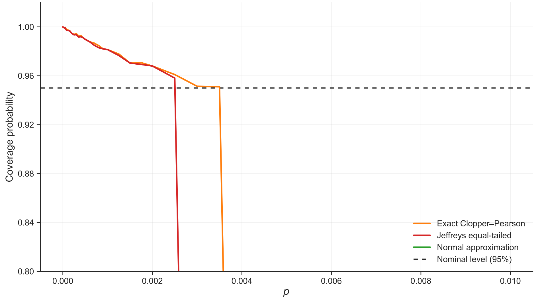
Coverage vs p ( n=1000 , \rho=0.15 )
