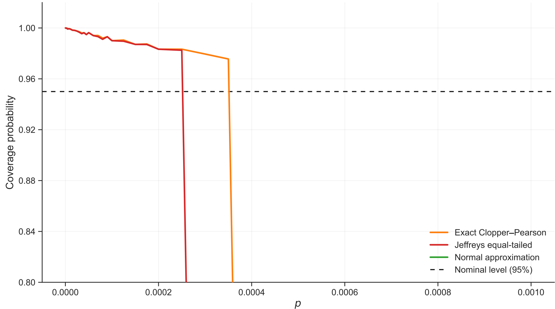
Coverage vs p (n=10000, rho=0.05)
