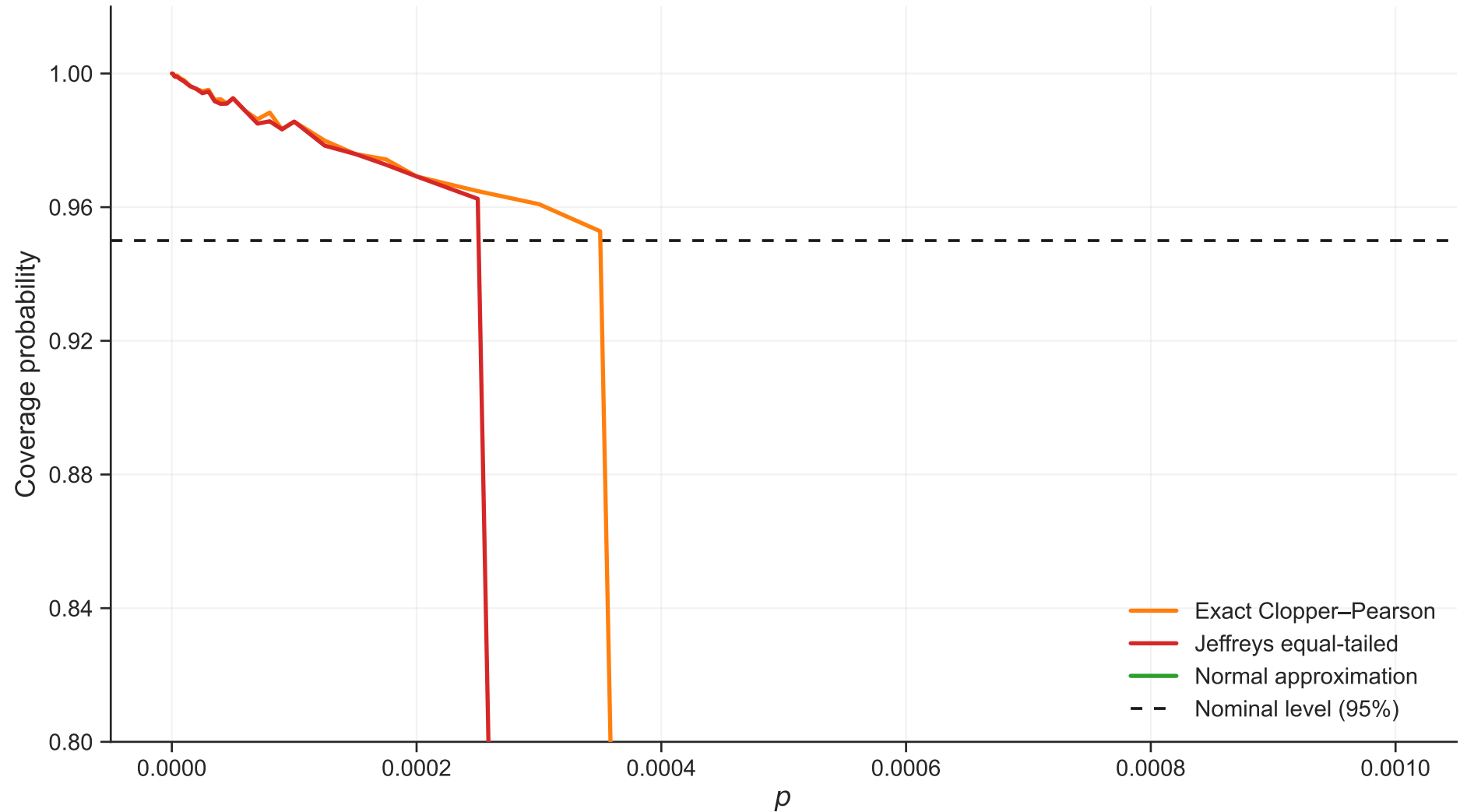
Coverage vs p (n=10000, rho=0.02)
