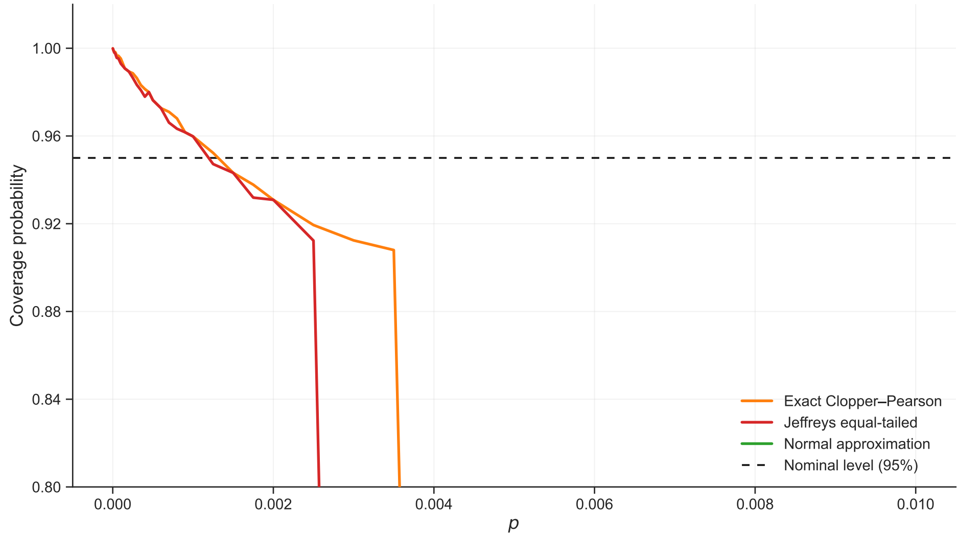
Coverage vs p ( n=1000 , \rho=0.05 )
