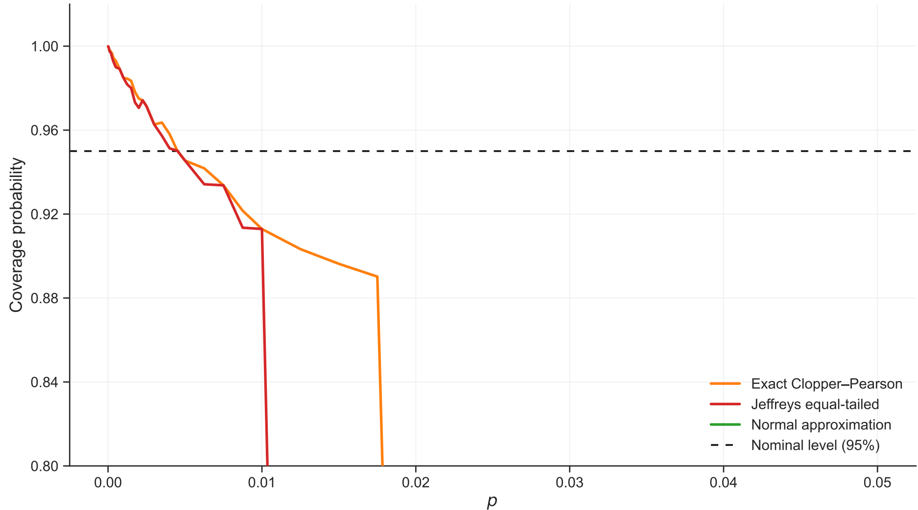
Coverage vs p (n=200, rho=0.15)
