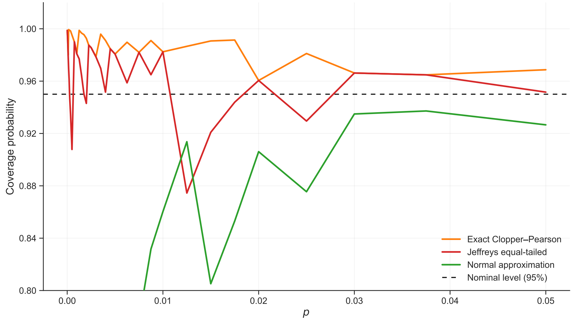
Coverage vs p ( n=200 , \rho=0.0 )
