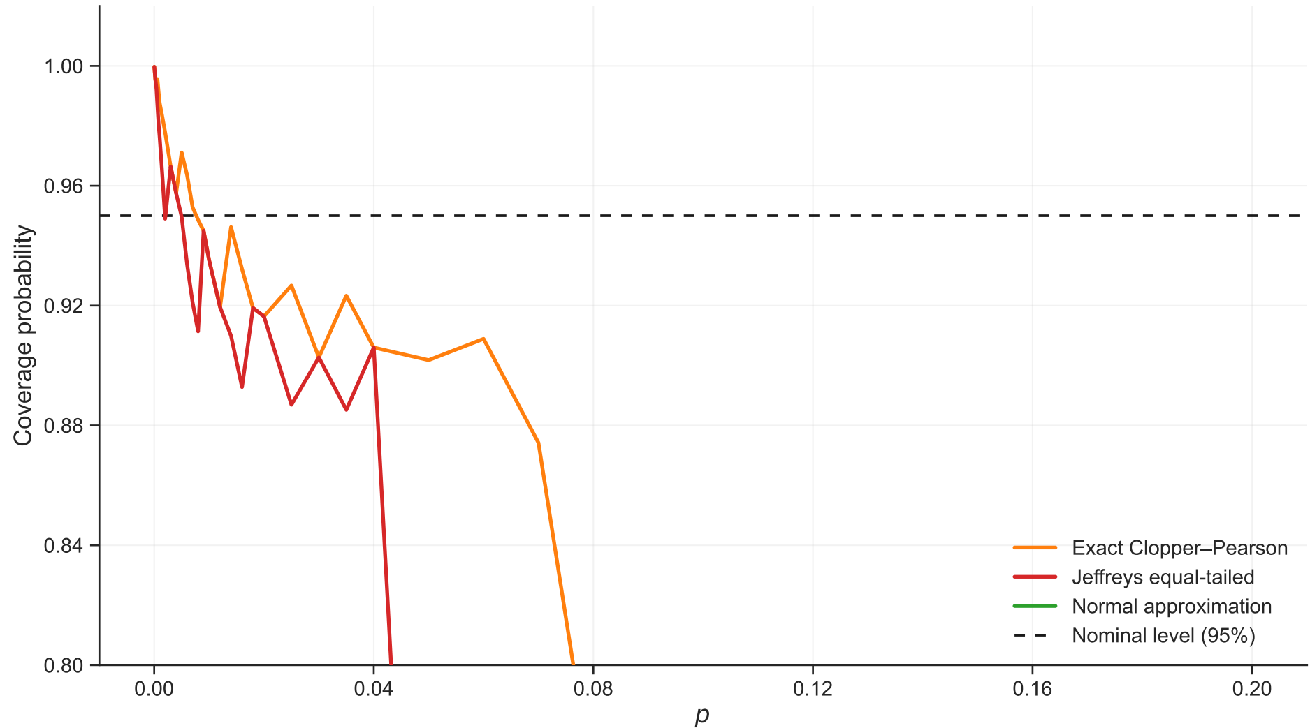
Coverage vs p ( n=50 , \rho=0.05 )
