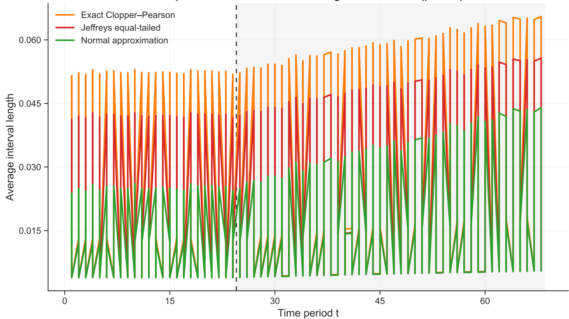
Temporal evolution of interval lengths under drift ( \hat{p}=0.01 )
