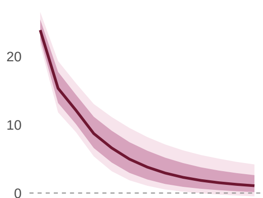
Geopolitical Risk (log)
