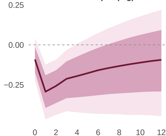
Real GDP p.c. (log)
