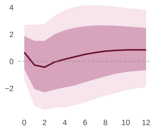
Real oil price (log)
