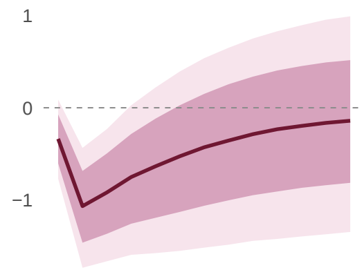
Investment p.c. (log)
