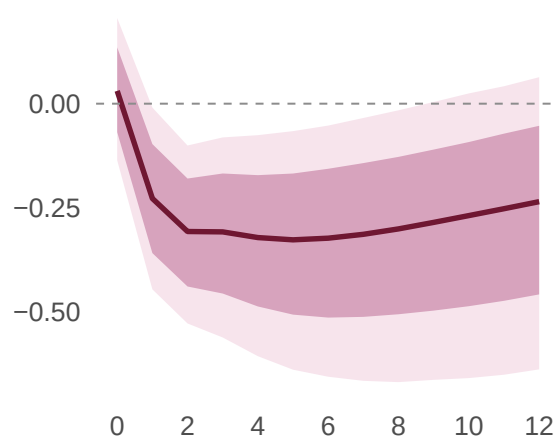
Private employment p.c. (log)
