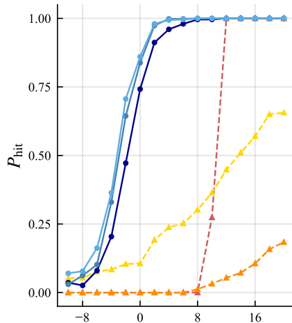
# True modes = 5
