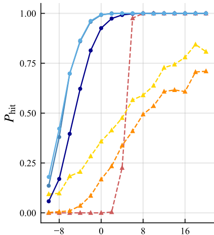
# True modes = 2
