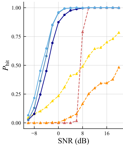
# True modes = 3
