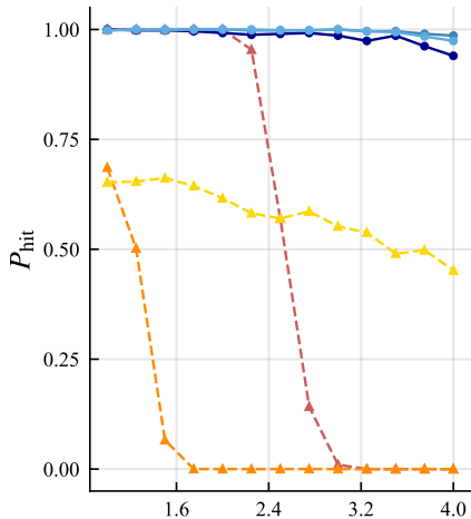
# True modes = 2
