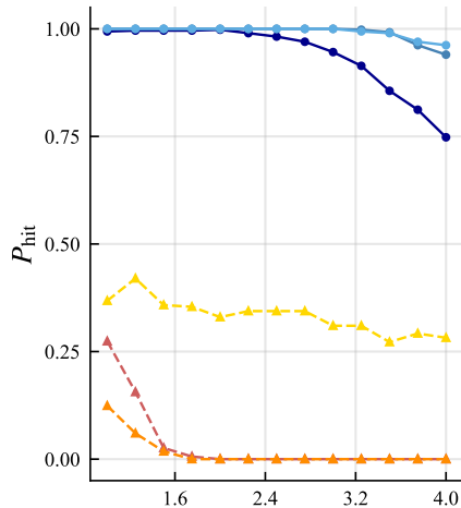
# True modes = 5
