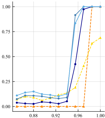
# True modes = 3
