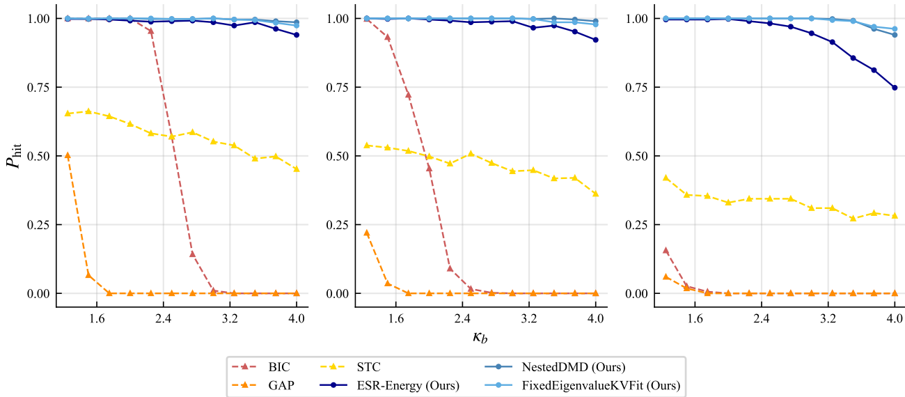
# True modes = 2
