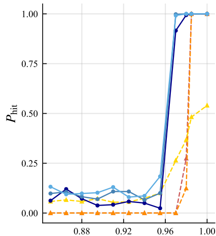
# True modes = 5
