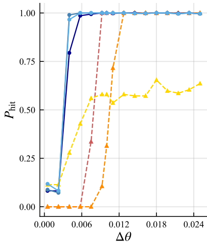
# True modes = 3
