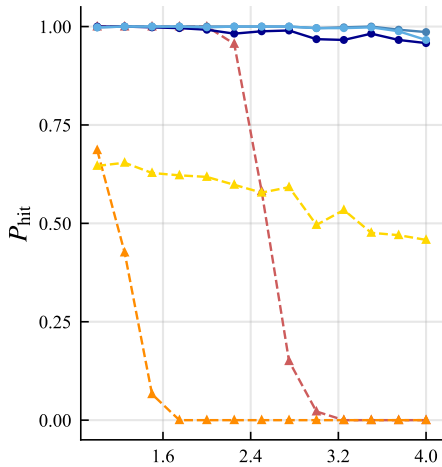
# True modes ( m ) = 2
