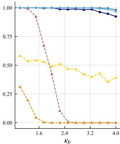
# True modes ( m ) = 3
