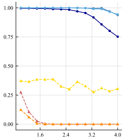
# True modes ( m ) = 5
